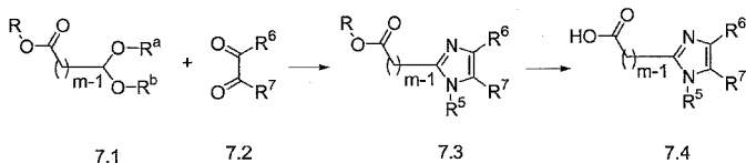
10 Scheme 7
