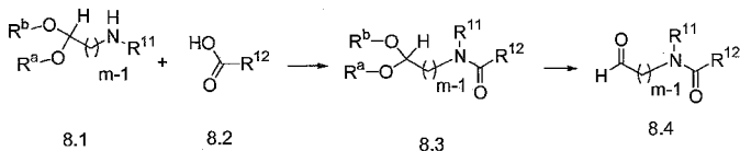
Scheme 8
