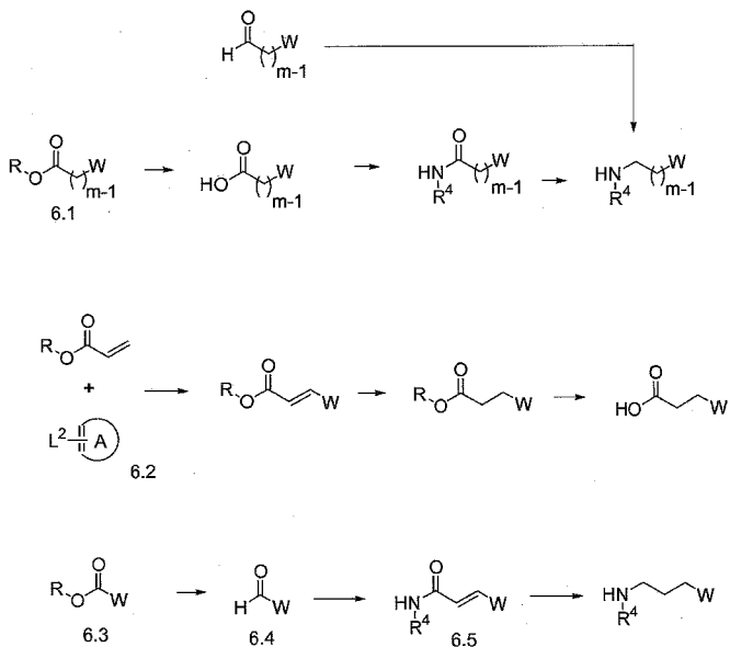
Scheme 6
