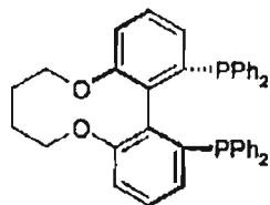
(R)-(+)-BINAP:
