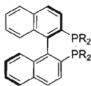
(R)-BINAP
