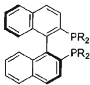
(S)-BINAP
