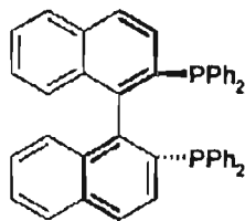
(R)-(+)-BINAP:
