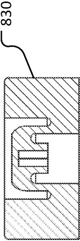
SECTION B-B
