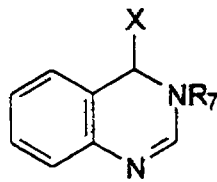
3,4-dihydro-quinazoline
