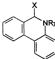
5,6-dihydro-phenanthridine
