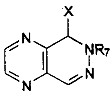
1,2-dihydro-pyrazino[2,3 d]pyridazine
