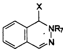
1,2-dihydro-phthalazine
