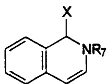
1,2-dihydro-isoquinoline
