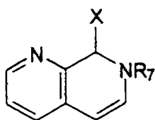
1,2-dihydro-pyrido[3,4b]pyridine
