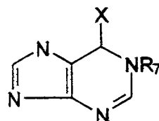
1,6-dihydro-purine
