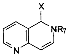
1,2-dihydro-pyrido[3,4b]pyridine
