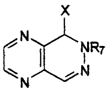
3,4-dihydro-pteridine
