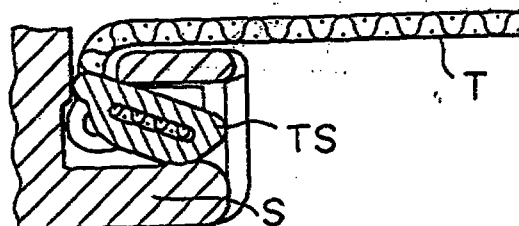
FIG. 8 PRIOR ART
