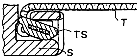
FIG. 8 PRIOR ART
