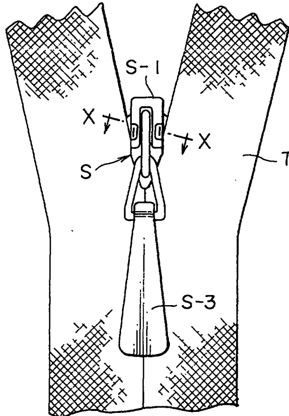
FIG. 7 PRIOR ART
