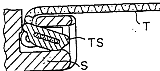
FIG. 8 PRIOR ART
