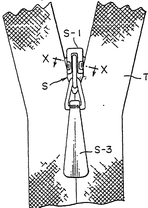
FIG. 7 PRIOR ART
