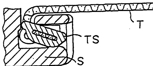
FIG. 8 PRIOR ART
