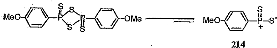
Scheme 14: The mechanism of catalysis for Lawesson's reagent.
