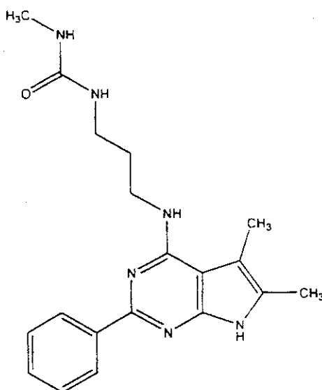
(Compound 1310)
