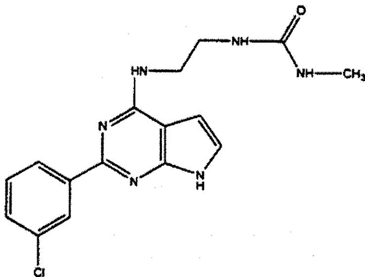
(Compound 1520)
