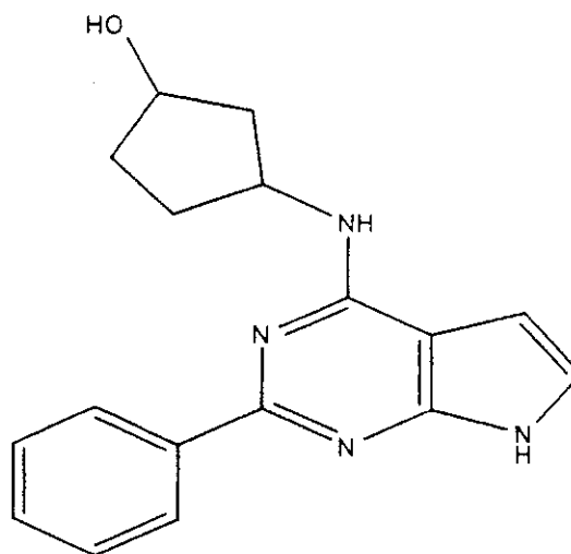
(Compound 1706) 15
