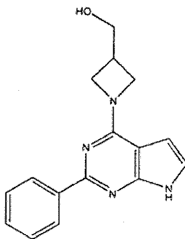
(Compound 1711)
