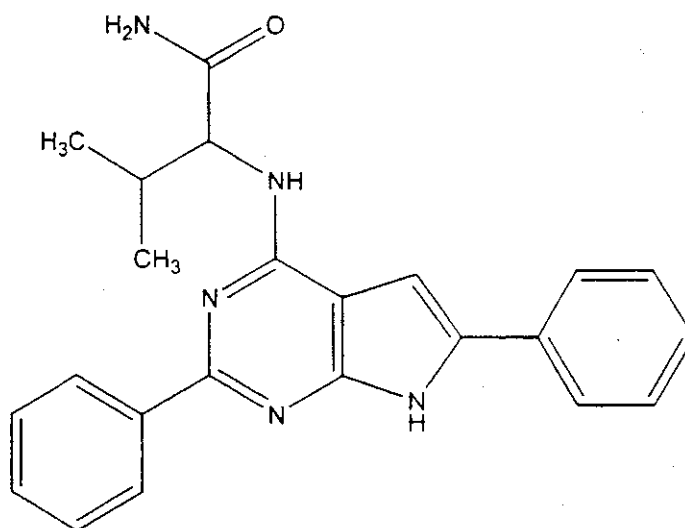
(Compound 1709)
