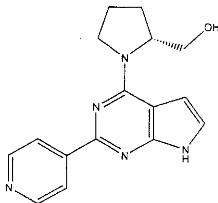
(Compound 1601)
