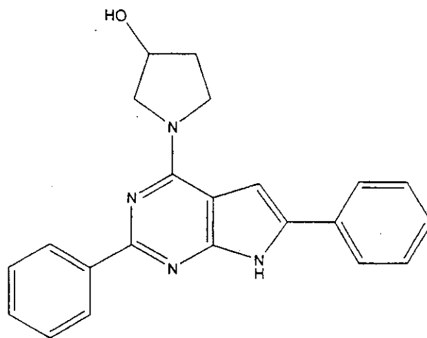
(Compound 1703)
