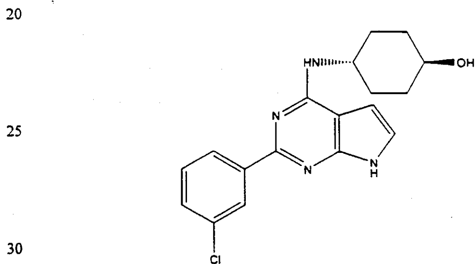
(Compound 1320)
