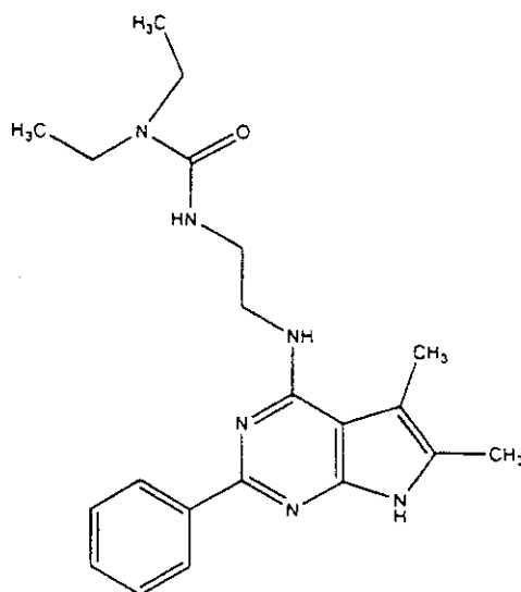
(Compound 1701)
