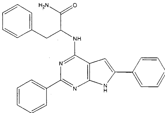
(Compound 1710)
