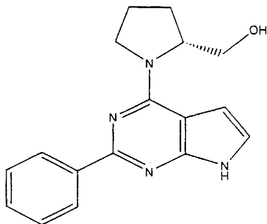
(Compound 1603)
