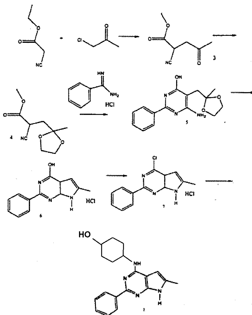
Scheme IV
