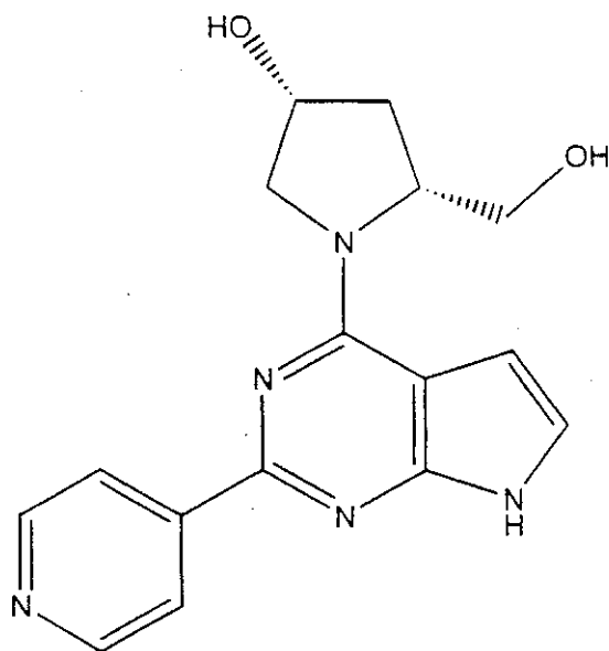
(Compound 1605)
