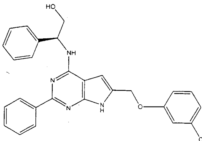
(Compound 1714)
