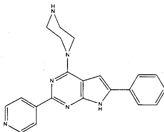
(Compound 1604)
