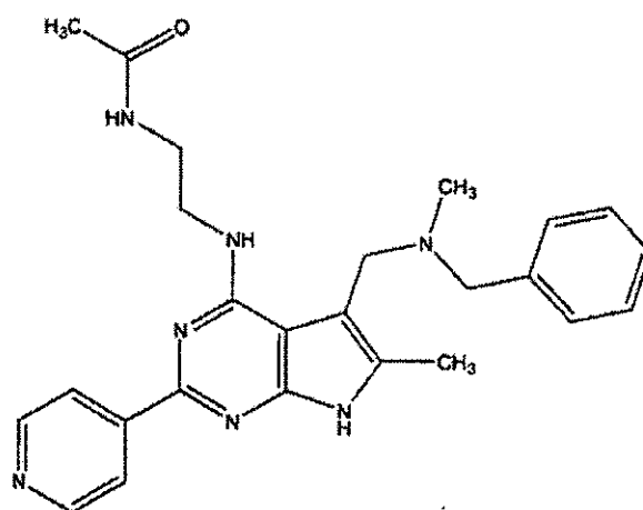
(Compound 1608)
