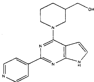
(Compound 1607)
