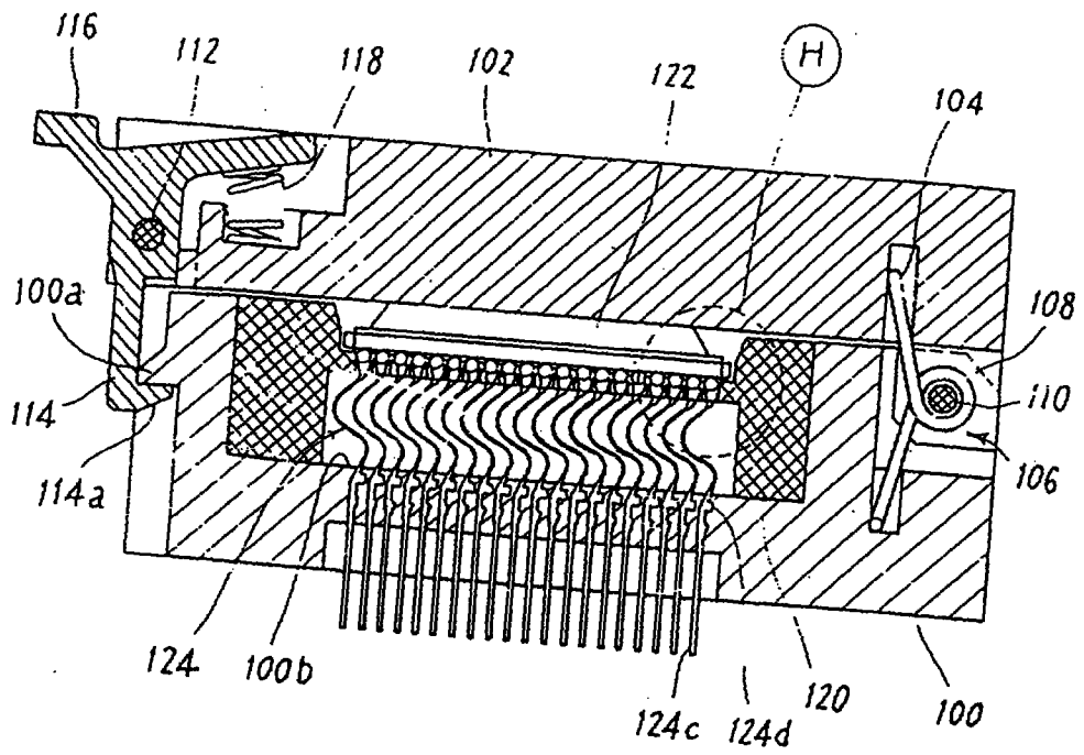
PRIOR ART FIG 35
