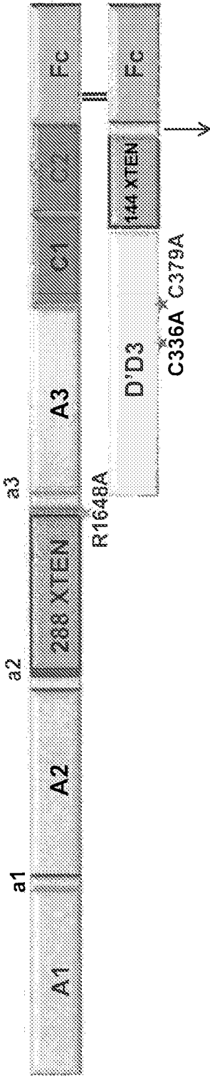
Bar diagram of representative FVIII-VWF heterodimer
