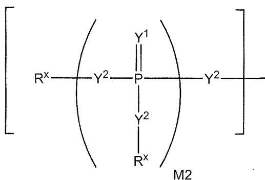
Formula Ia
