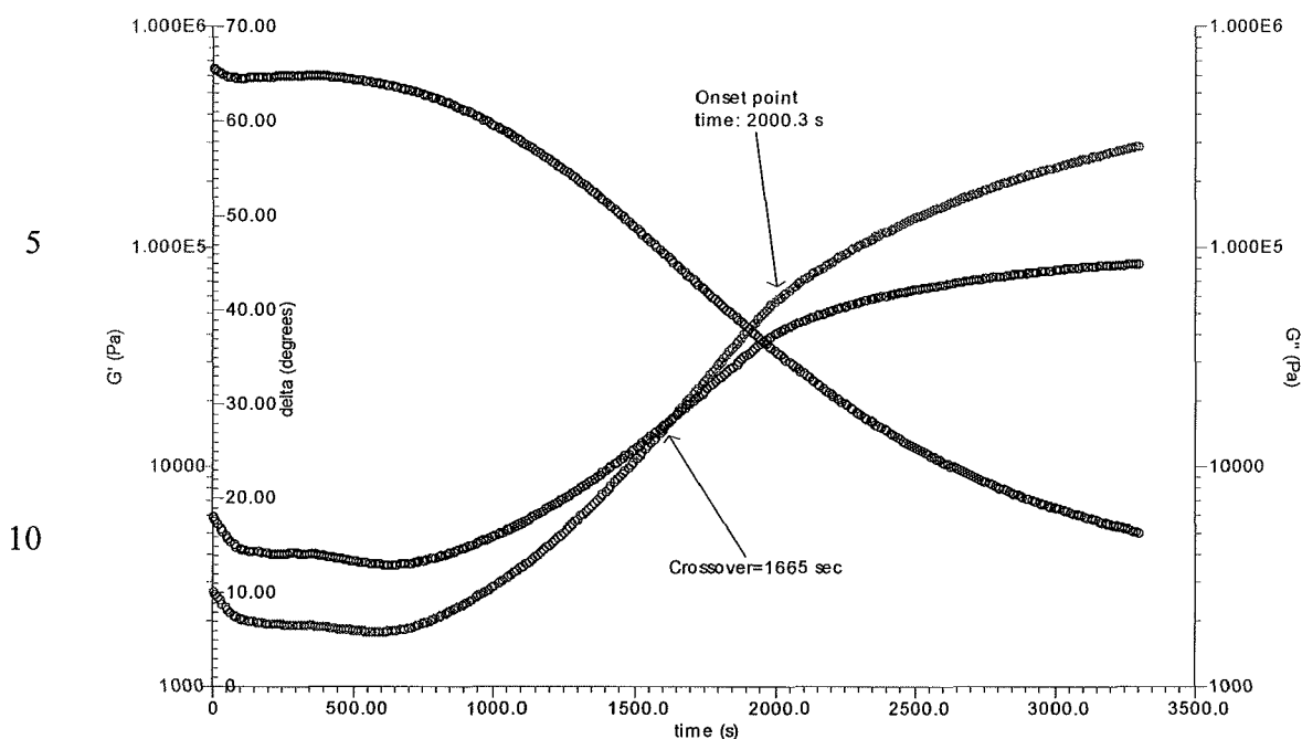
15 Graph 1. Parallel Plate Rheology of Blend 3, at 380 °C. See, J. Mercel et al. , "Thermal Analysis of Polymers: Fundamentals and Applications," p. 445, Wiley, ed. 1 (2009).
