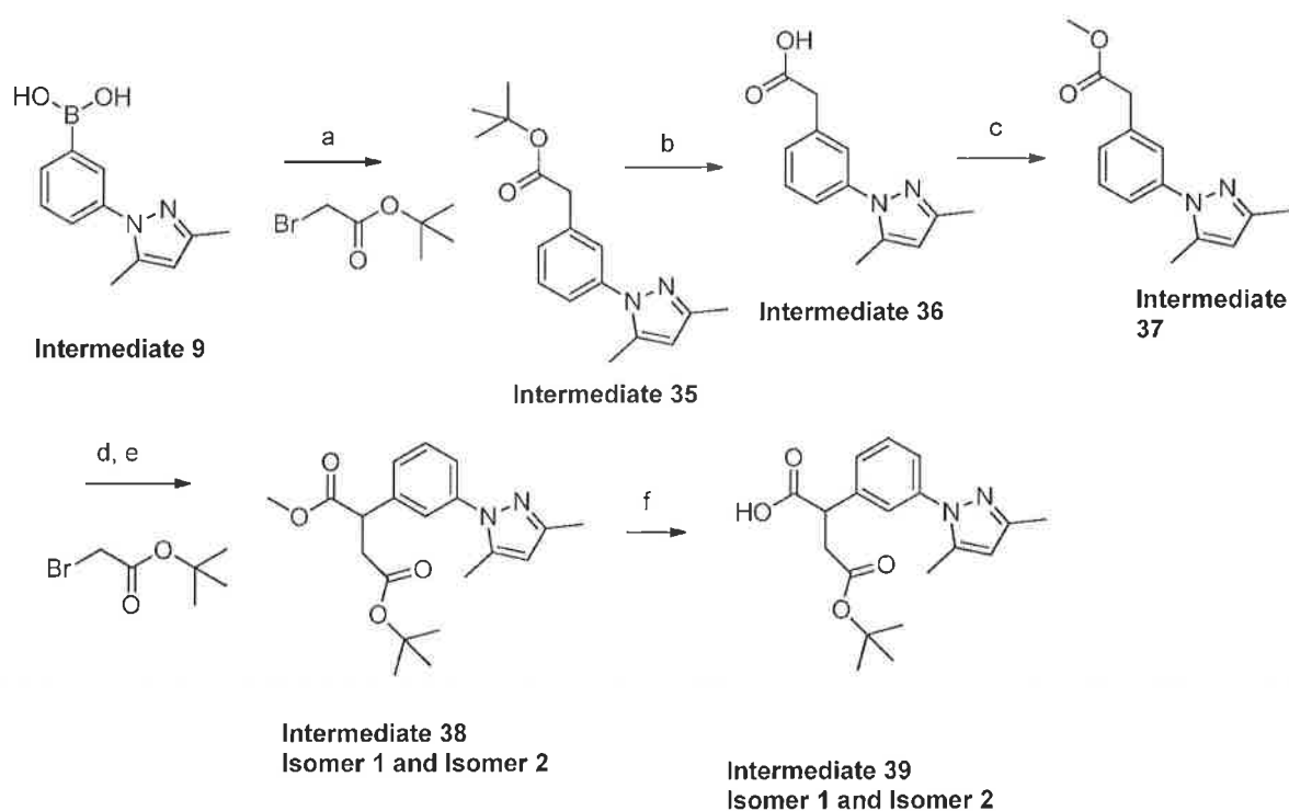
Scheme 4 Reagents and Conditions: (a) \text{Pd}(\text{OAc})_2 , \text{P}(\text{o-tolyl})_3 , \text{K}_3\text{PO}_4 , THF, reflux; (b) TFA, DCM; (c) MeOH, HCl, reflux; (d) \text{LiN}(\text{TMS})_2 , THF, -78^\circ\text{C} ; (e) Preparative chiral HPLC separation; (f) \text{LiOH} , \text{H}_2\text{O}_2 , THF, 0^\circ\text{C}
