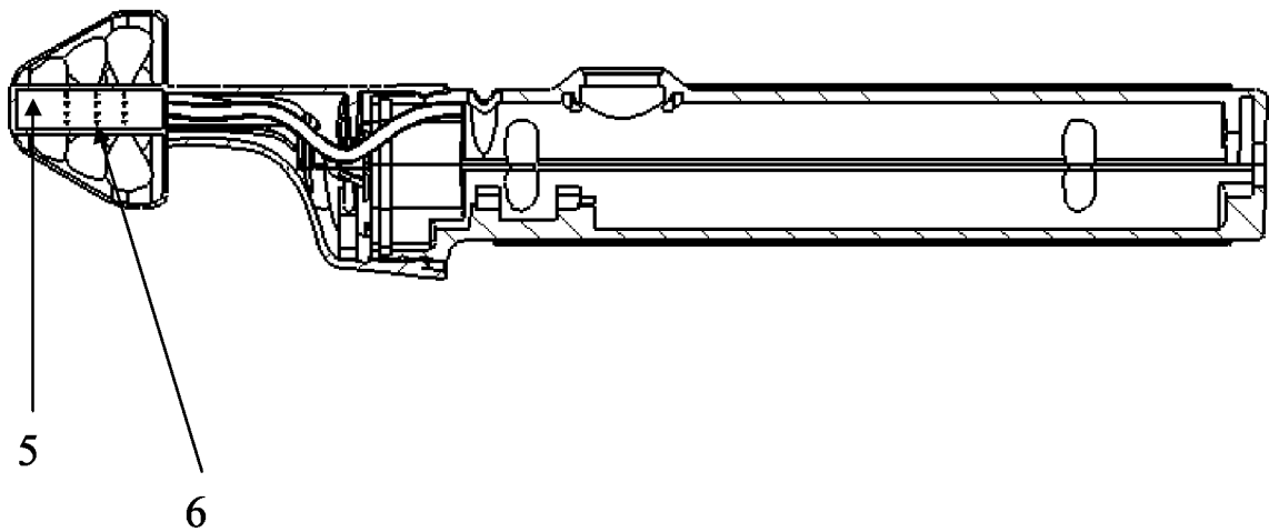
Figure 3B Cross-section A-A
