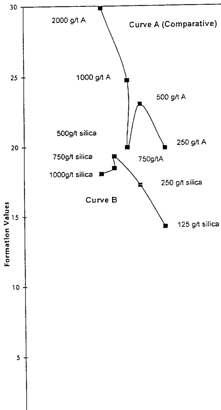
Figure 1 Formation-Drainage Curve
