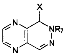
1,2-dihydro-pyrazino[2,3d]pyridazine
