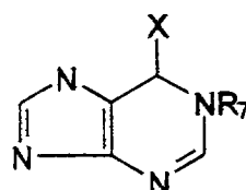
1,6-dihydro-purine
