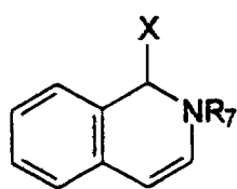
1,2-dihydro-isoquinoline
