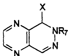
3,4-dihydro-pteridine
