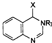
3,4-dihydro-quinazoline
