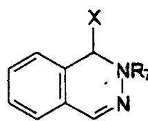
1,2-dihydro-phthalazine
