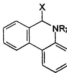
5,6-dihydro-phenanthridine
