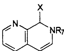
1,2-dihydro-pyrido[3,4b]pyridine
