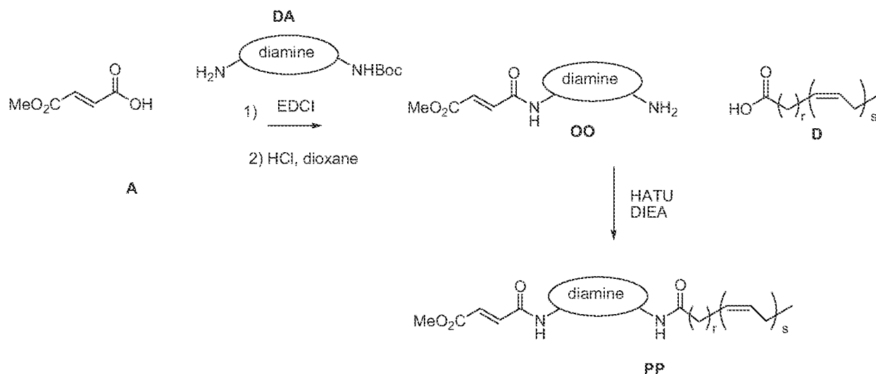
Scheme 11
