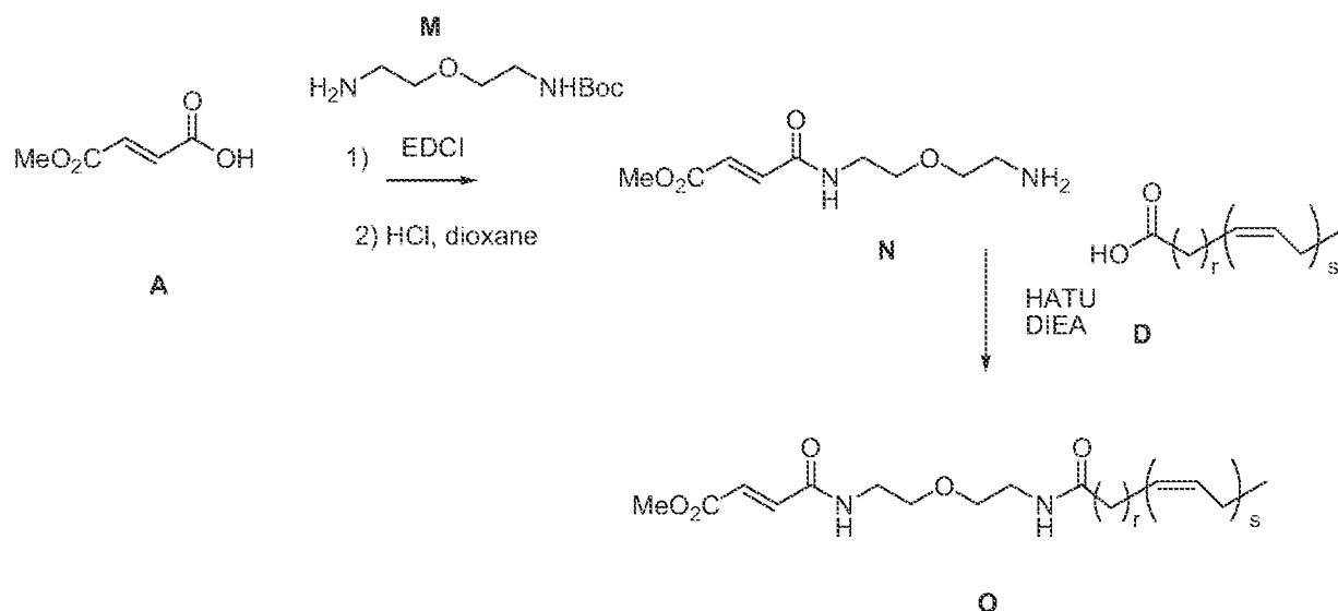
Scheme 4
