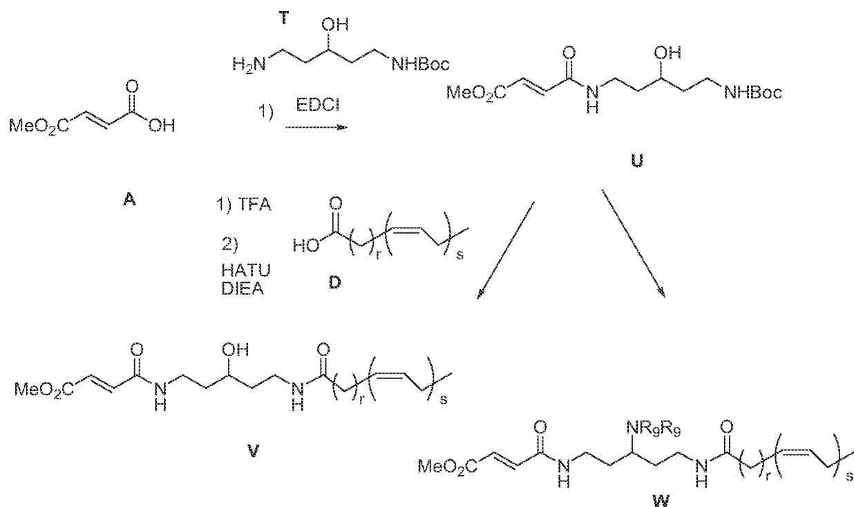
Scheme 6
