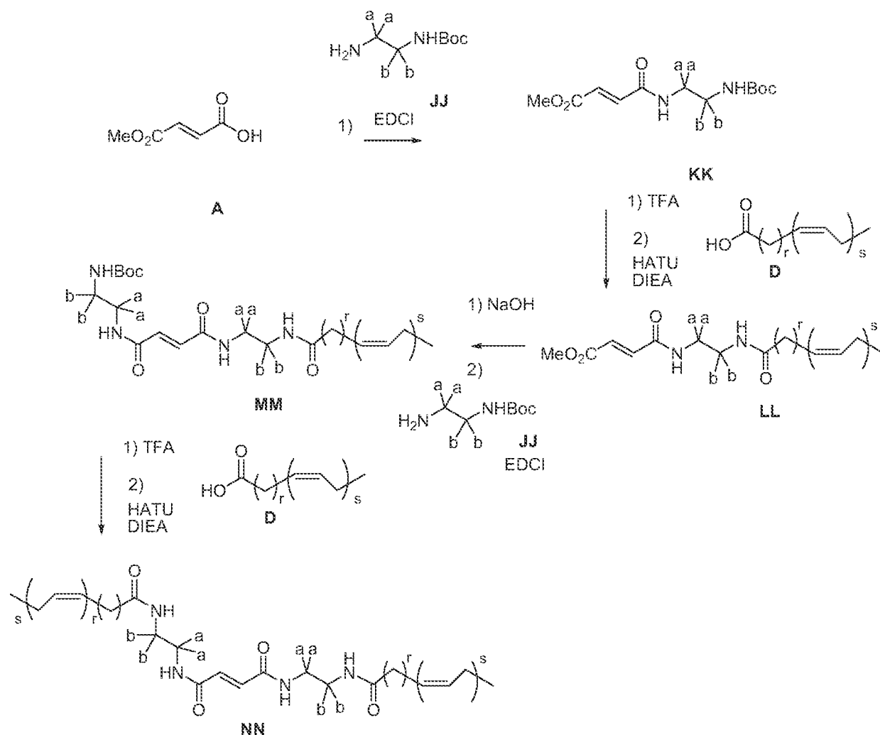
Scheme 10
