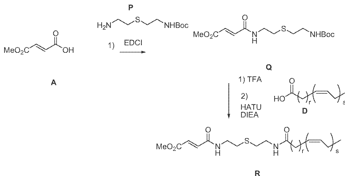
Scheme 5
