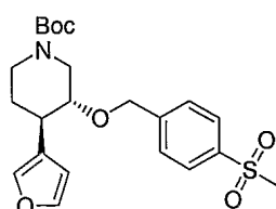
4-Furan-3-yl-3-(4-methanesulfonyl-benzyloxy)-piperidine-1-carboxylic acid tert -butyl ester, 98 , Exact Mass: 435.1716
