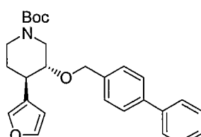
3-(Biphenyl-4-ylmethoxy)-4-furan-3-yl-piperidine-1-carboxylic acid tert -butyl ester, 89 , Exact Mass: 433.2253
