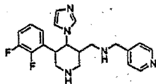
[5-(2,3-Difluoro-phenyl)-4-imidazol-1-yl-piperidin-3-ylmethyl]-pyridin-4-ylmethyl-amine
