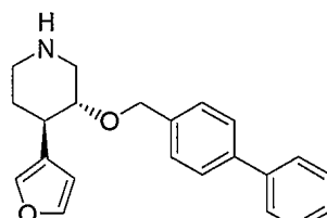
3-(Biphenyl-4-ylmethoxy)-4-furan-3-yl-piperidine, 105 , Exact Mass: 333.1729
