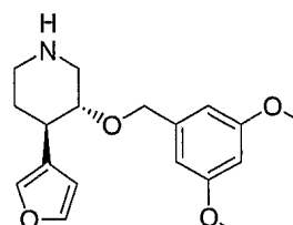
3-(3,5-Dimethoxy-benzyloxy)-4-furan-3-yl-piperidine, 112 , Exact Mass: 317.1627
