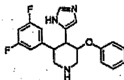
3-(3,5-Difluoro-phenyl)-4-(3H-imidazol-4-yl)-5-phenoxy-piperidine
