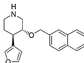
4-Furan-3-yl-3-(naphthalen-2-ylmethoxy)-piperidine, 106 , Exact Mass: 307.1572
