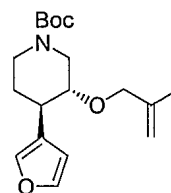
4-Furan-3-yl-3-(2-methyl-allyloxy)-piperidine-1-carboxylic acid tert -butyl ester, 99 , Exact Mass: 321.1940
