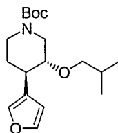
4-Furan-3-yl-3-isobutoxy-piperidine-1-carboxylic acid tert -butyl ester, 102 , Exact Mass: 323.2097
