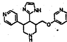
4-(1H-imidazol-2-yl)-5-(pyridin-3-ylloxymethyl)-1,2,3,4,5,6-hexahydro-[3,4']bipyridinyl
