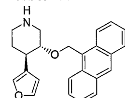
3-(Anthracen-9-ylmethoxy)-4-furan-3-yl-piperidine, 110 , Exact Mass: 357.1729
