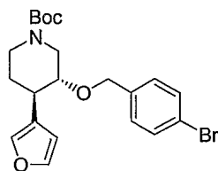
3-(4-Bromo-benzyloxy)-4-furan-3-yl-piperidine-1-carboxylic acid tert -butyl ester, 97 , Exact Mass: 435.1045
