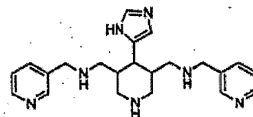
4-(3H-imidazol-4-yl)-5-(((pyridin-3-ylmethyl)-amino)-methyl)-piperidin-3-ylmethyl-pyridin-3-ylmethyl-amine
