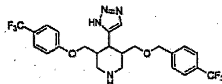
4-(3H-[1,2,3]Triazol-4-yl)-3-(4-trifluoromethyl-benzoyloxymethyl)-5-(4-trifluoromethyl-phenoxy-methyl)-piperidine
