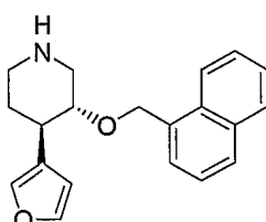
4-Furan-3-yl-3-(naphthalen-1-ylmethoxy)-piperidine, 107 , Exact Mass: 307.1572
