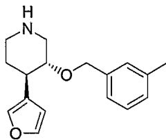
4-Furan-3-yl-3-(3-methylbenzyloxy)-piperidine, 111 , Exact Mass: 271.1572
