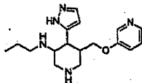
Propyl-[4-(2H-pyrazol-3-yl)-5-(pyridin-3-ylmethoxymethyl)-piperidin-3-yl]-amine
