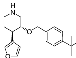
3-(4- tert -Butyl-benzyloxy)-4-furan-3-yl-piperidine, 109 , Exact Mass: 313.2042
