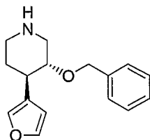
3-Benzyloxy-4-furan-3-yl-piperidine, 104 , Exact Mass: 257.1416
