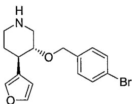
3-(4-Bromo-benzyloxy)-4-furan-3-yl-piperidine, 113 , Exact Mass: 335.0521
