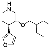
3-(2-Ethyl-butoxy)-4-furan-3-yl-piperidine, 118 , Exact Mass: 251.1885
