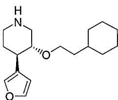
3-(2-Cyclohexyl-ethoxy)-4-furan-3-yl-piperidine, 116 , Exact Mass: 277.2042
