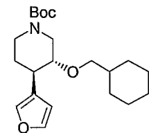
3-Cyclohexylmethoxy-4-furan-3-yl-piperidine-1-carboxylic acid tert -butyl ester, 100 , Exact Mass: 363.2410
