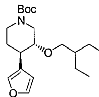
3-(2-Ethyl-butoxy)-4-furan-3-yl-piperidine-1-carboxylic acid tert -butyl ester, 103 , Exact Mass: 351.4804
