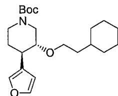
3-(2-Cyclohexyl-ethoxy)-4-furan-3-yl-piperidine-1-carboxylic acid tert -butyl ester, 101 , Exact Mass: 377.2566
