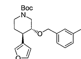
4-Furan-3-yl-3-(3-methylbenzyloxy)-piperidine-1-carboxylic acid tert -butyl ester, 95 , Exact Mass: 371.2097
