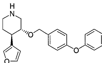
4-Furan-3-yl-3-(4-phenoxybenzyloxy)-piperidine, 108 , Exact Mass: 349.1678
