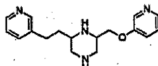
2-(2-Pyridin-3-yl-ethyl)-6-(pyridin-3-yloxymethyl)-piperazine
