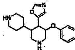
4-Oxazol-5-yl-5-phenoxy-(3,4'-bipiperidinyl)
