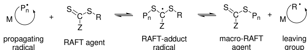
Scheme 1: Proposed mechanism for RAFT polymerisation.
