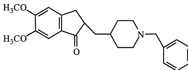
Compound (R)
