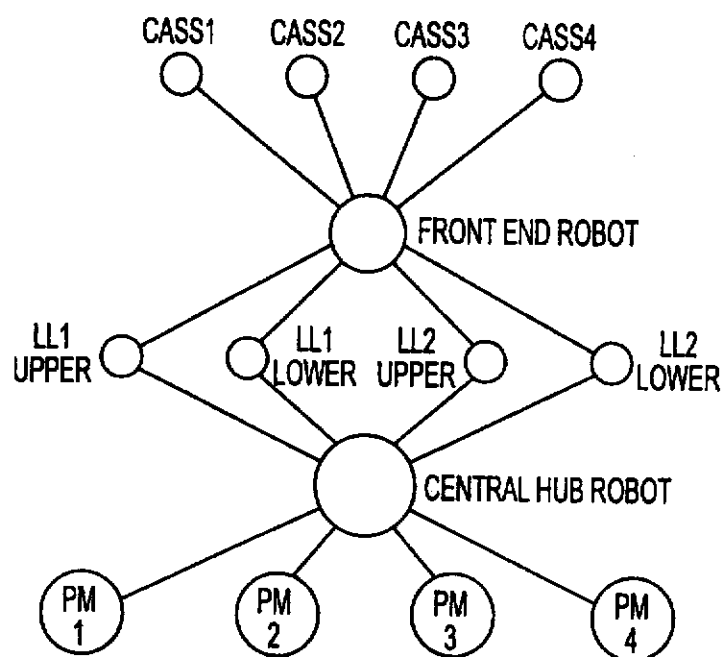
FIG. 4 (PRIOR ART)
