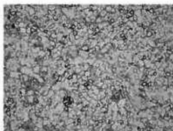
Comparative Example 8 (Forging Temperature 400 °C, \Delta \varepsilon = 9 )
