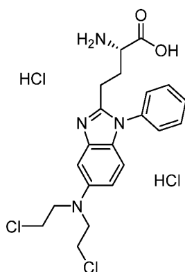
Scheme 11
