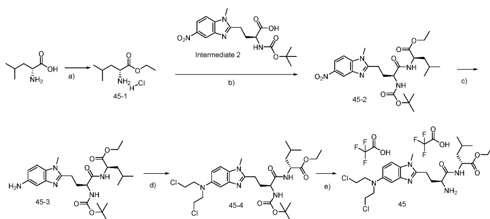
Scheme 12
