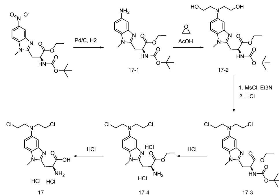
Scheme 6
