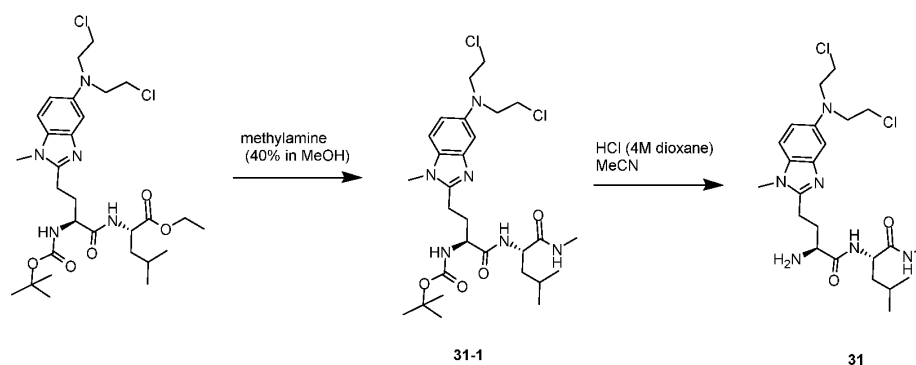
Scheme 9
