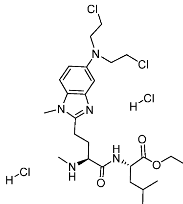
Scheme 10
