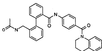
compound B
