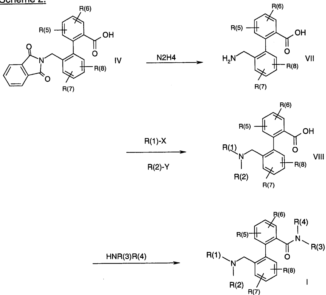
Scheme 2:
