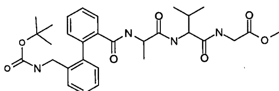
compound A
