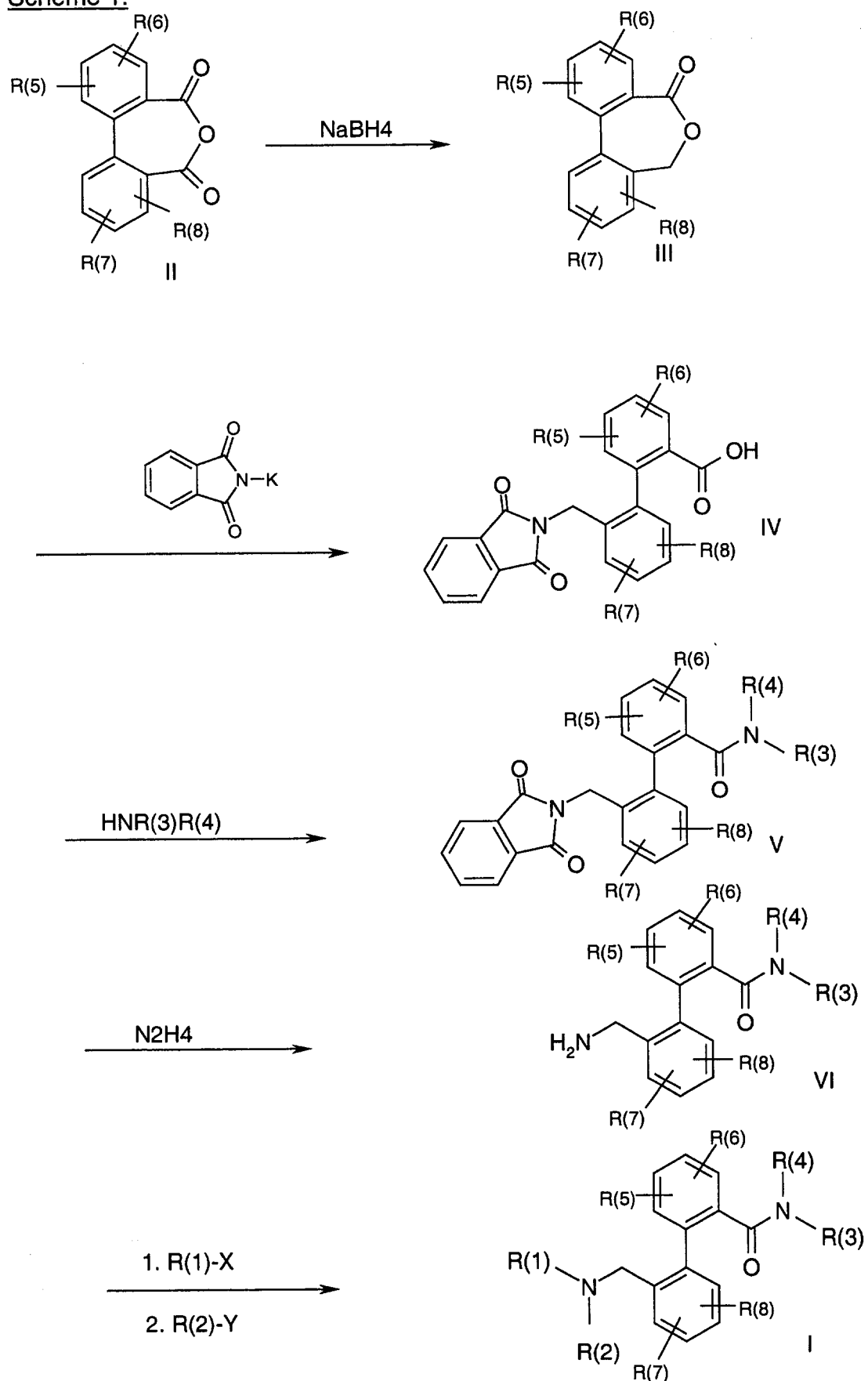
Scheme 1:
