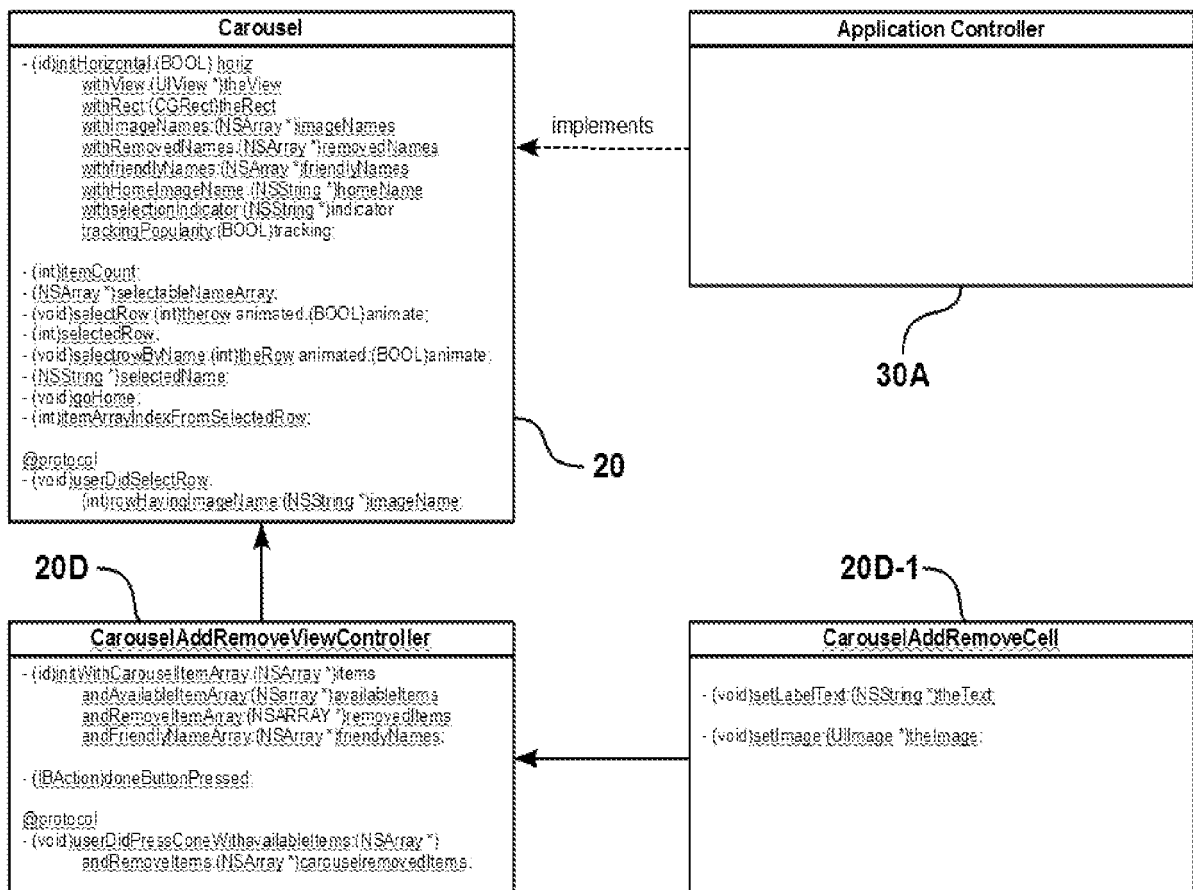
Class Diagram for CSC Carousel
