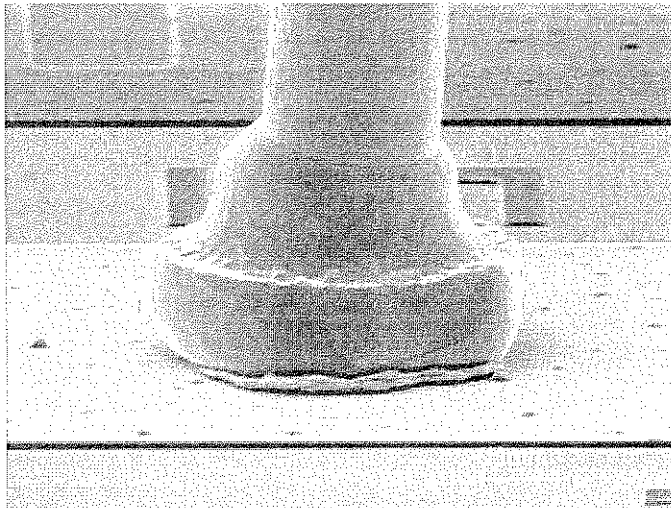
Fig 3(b) – Ball bond of 1N secondary alloyed Cu 0.8mil wire
