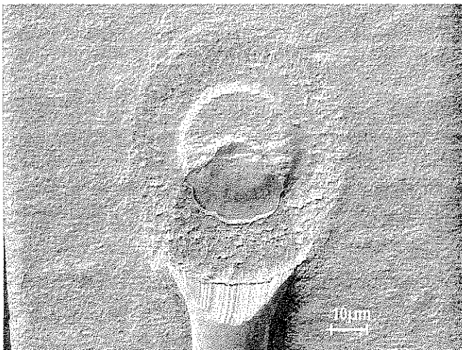
Fig 3(c) – Stitch bond of 1N secondary alloyed Cu 0.8mil wire
