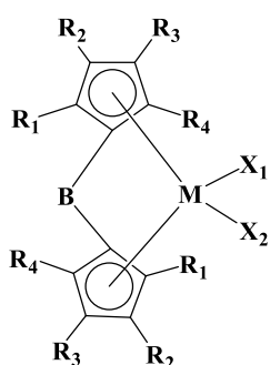
[Chemical Formula 2]
