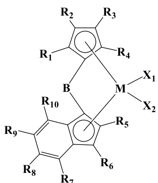
[Chemical Formula 3]
