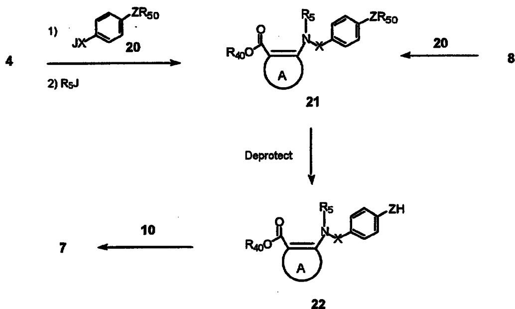
Scheme 5:
