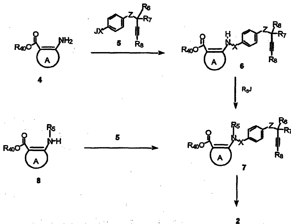
Scheme 2:
