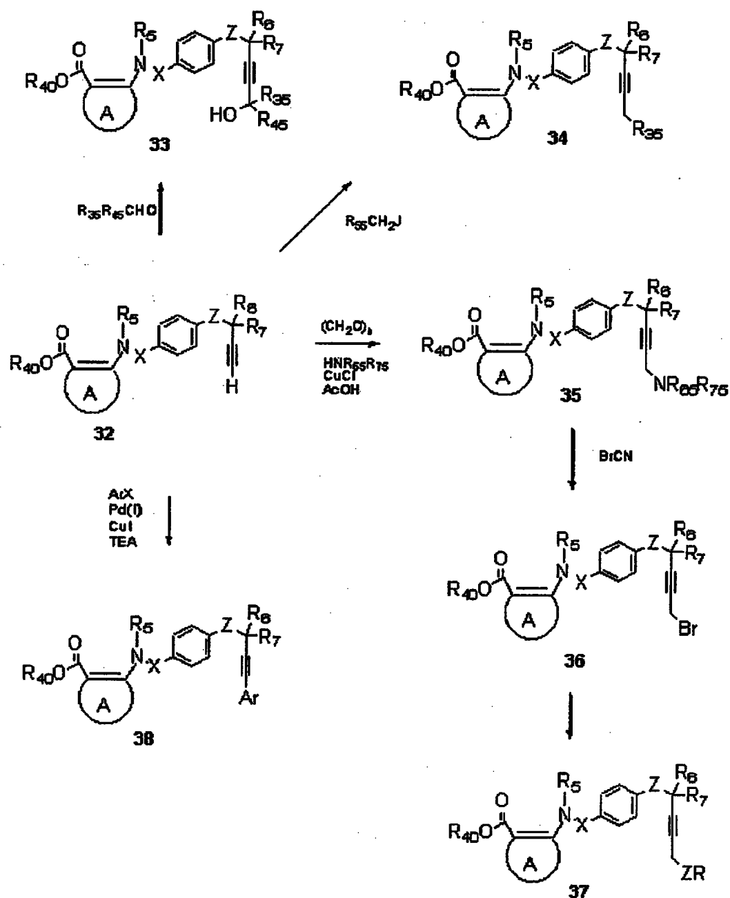
Scheme 9:
