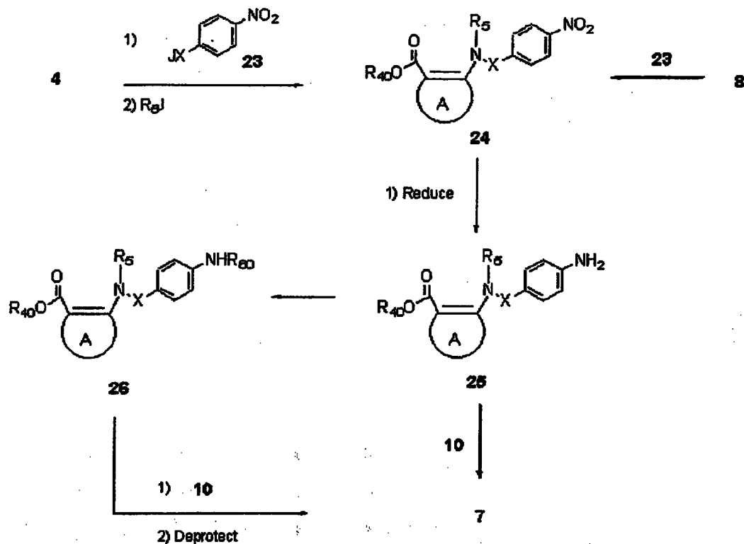
Scheme 6:
