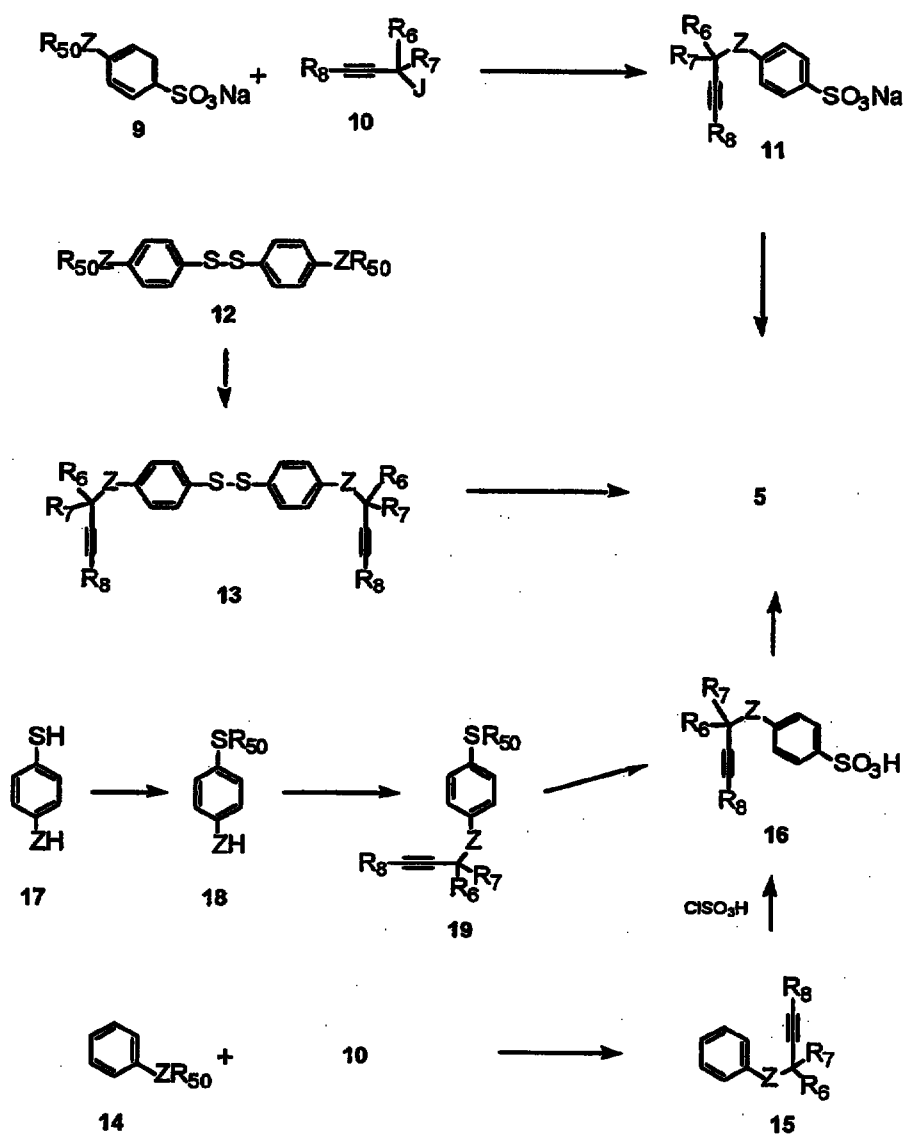
Scheme 3:
