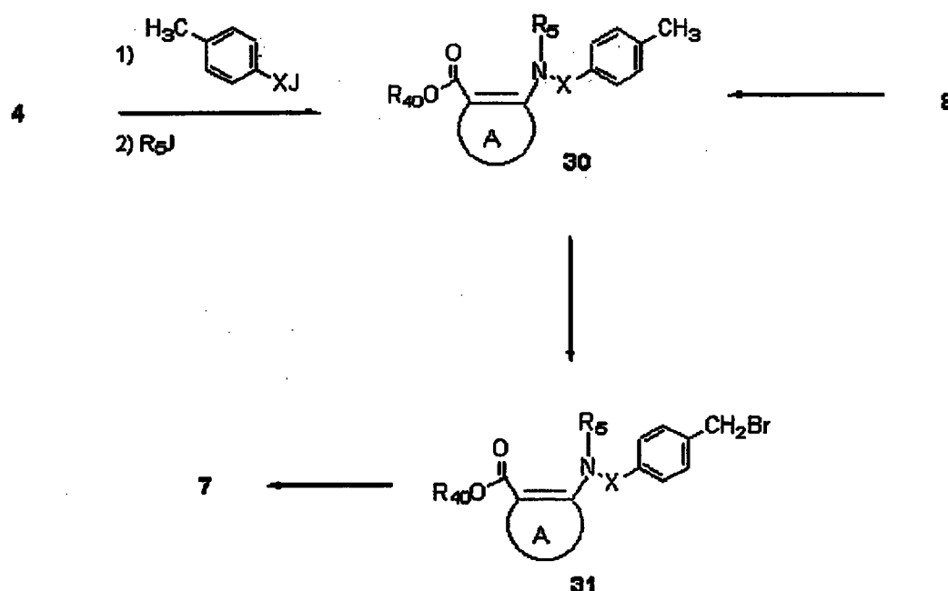
Scheme 8:
