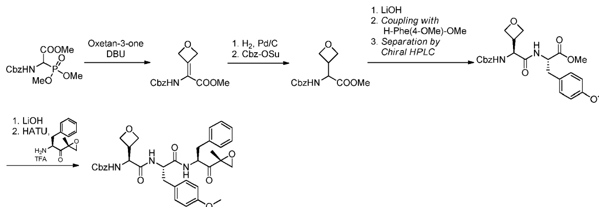
Methyl 2-(benzyloxycarbonylamino)-2-(oxetan-3-ylidene)acetate
