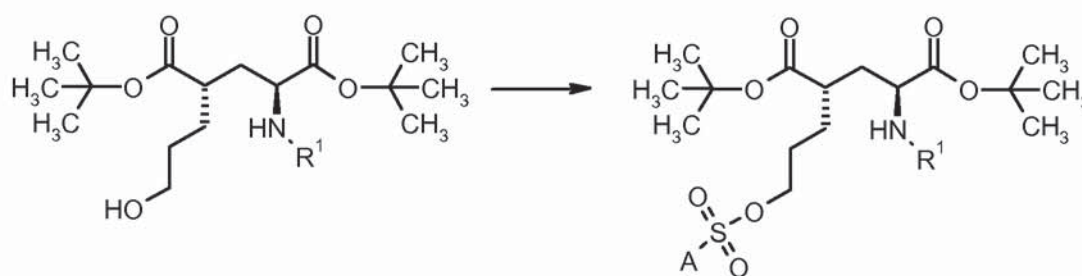
Formula Ia
