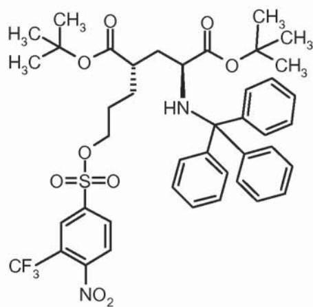
Di-tert-butyl (4S)-4-[3-({[4-nitro-3-(trifluoromethyl)phenyl]sulfonyl}oxy)propyl]-N-trityl-L-glutamate
