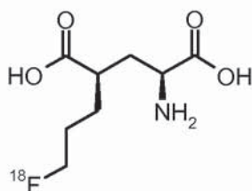
Formula IVb-F18
