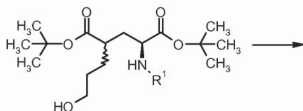
Formula IIa/b
