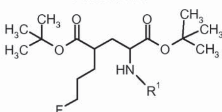
Formula III-F
