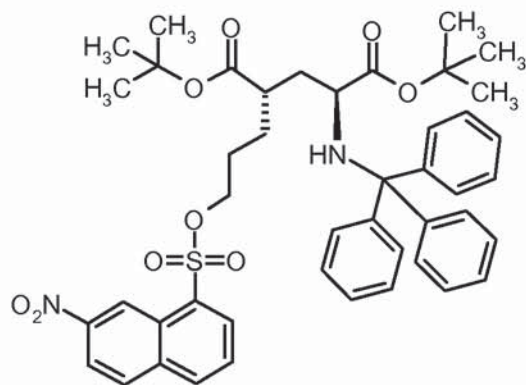
Di-tert-butyl (4S)-4-(3-[(7-nitro-1-naphthyl)sulfonyl]oxy)propyl-N-trityl-L-glutamate
