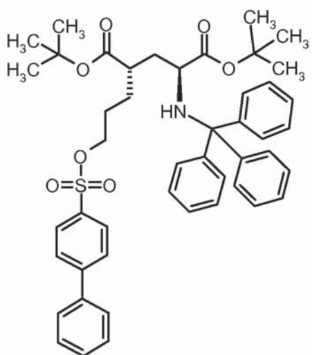
Di-tert-butyl (4S)-4-{3-[(biphenyl-4-ylsulfonyl)oxy]propyl}-N-trityl-L-glutamate
