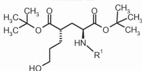
Formula IIa
