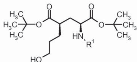
Formula IIb
