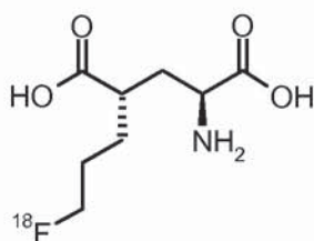
Formula IVa-F18
