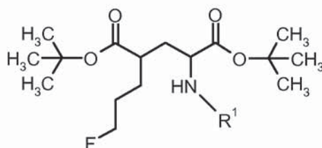
Formula III-F
