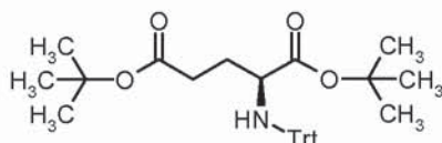
di- tert -butyl N -trityl-L-glutamate
