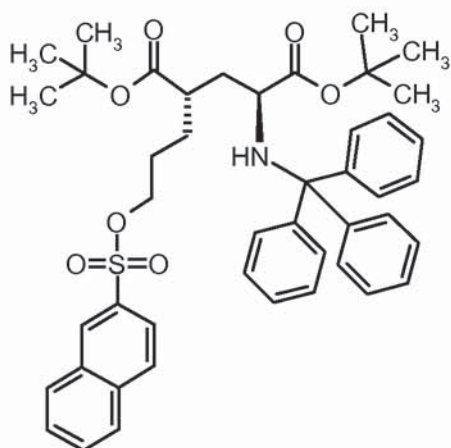
Di-tert-butyl (4S)-4-{3-[(2-naphthylsulfonyl)oxy]propyl}-N-trityl-L-glutamate
