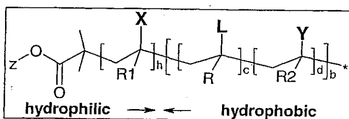
FORMULA (VI)
