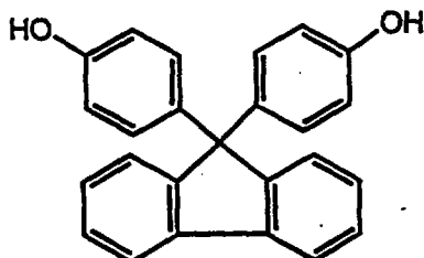
K - 9,9-bis(4-hydroxyphenyl)fluorene
