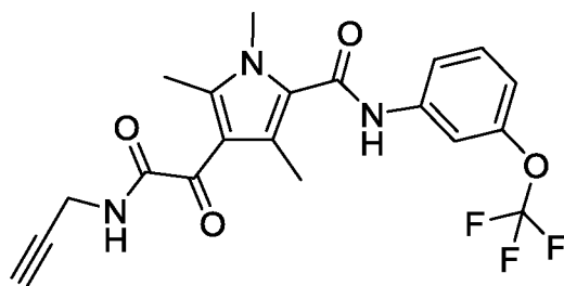
1,3,5-trimethyl-4-(2-oxo-2-(prop-2-yn-1-ylamino)acetyl)-N-(3-(trifluoromethoxy)phenyl)-1H-pyrrole-2-carboxamide ( 55 )
