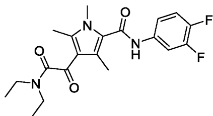
4-(2-(diethylamino)-2-oxoacetyl)-N-(3,4-difluorophenyl)-1,3,5-trimethyl-1H-pyrrole-2-carboxamide (45)
