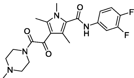
N-(3,4-difluorophenyl)-1,3,5-trimethyl-4-(2-(4-methylpiperazin-1-yl)-2-oxoacetyl)-1H-pyrrole-2-carboxamide ( 44 )
