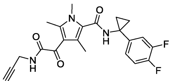
N-(1-(3,4-difluorophenyl)cyclopropyl)-1,3,5-trimethyl-4-(2-oxo-2-(prop-2-yn-1-ylamino)acetyl)-1H-pyrrole-2-carboxamide (57)
