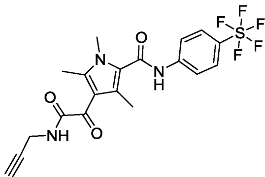
1,3,5-trimethyl-4-(2-oxo-2-(prop-2-yn-1-ylamino)acetyl)-N-(4-(pentafluorosulfanyl)phenyl)-1H-pyrrole-2-carboxamide (59)
