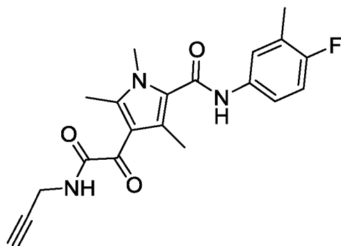
N-(4-fluoro-3-methylphenyl)-1,3,5-trimethyl-4-(2-oxo-2-(prop-2-yn-1-ylamino)acetyl)-1H-pyrrole-2-carboxamide (64)
