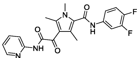
N-(3,4-difluorophenyl)-1,3,5-trimethyl-4-(2-oxo-2-(pyridin-2-ylamino)acetyl)-1H-pyrrole-2-carboxamide ( 43 )
