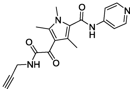
1,3,5-trimethyl-4-(2-oxo-2-(prop-2-yn-1-ylamino)acetyl)-N-(pyridin-4-yl)-1H-pyrrole-2-carboxamide (63)
