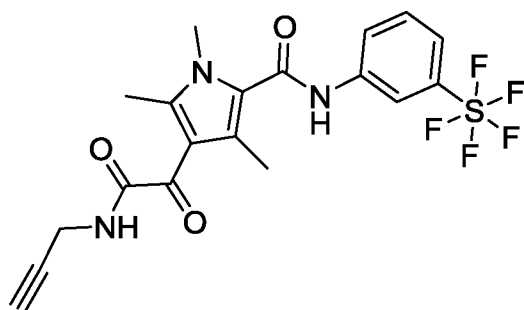
1,3,5-trimethyl-4-(2-oxo-2-(prop-2-yn-1-ylamino)acetyl)-N-(3-(pentafluorosulfanyl)phenyl)-1H-pyrrole-2-carboxamide (60)
