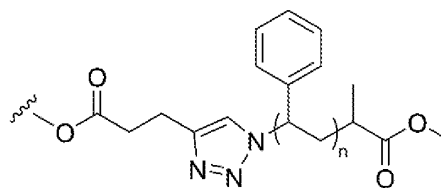
(IIIId)
