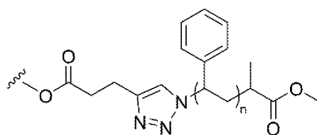
(IIIc)
