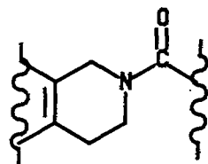
Amides
