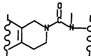
Ureas
