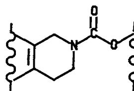
Carbamate
