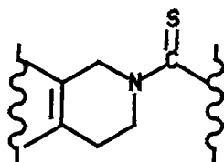
Thioamides
