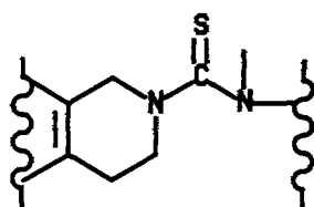
Thioureas
