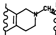
N-alkyls
