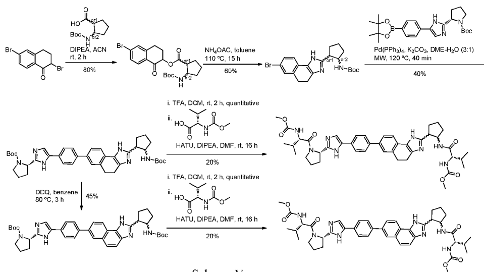
Scheme V
