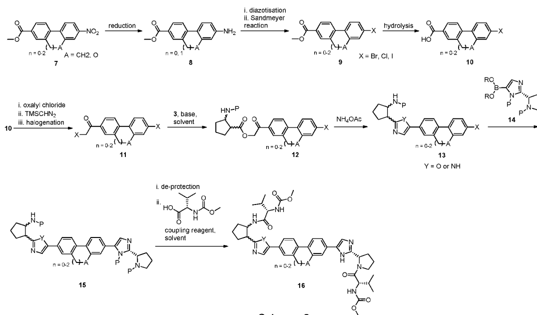
Scheme 2
