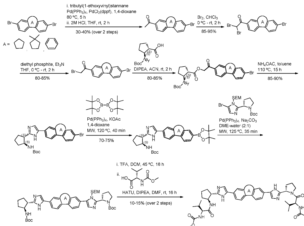
Scheme VII
