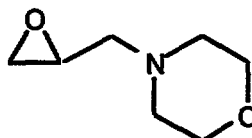
4-(2,3-Epoxypropyl) morpholine
