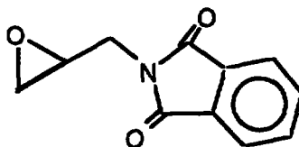
N-(2,3-Epoxypropyl)-phthalimide
