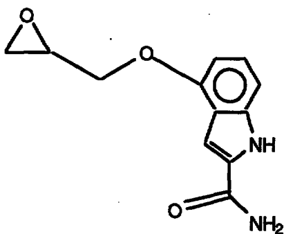
4-Glycidyloxy-2-Indole carboxamide
