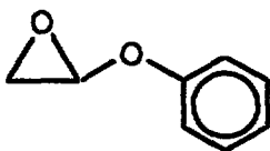
(±)-1,2-Epoxy-3-phenoxypropane
