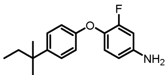
3-Fluoro-4-(4-(tert-pentyl)phenoxy)aniline,
