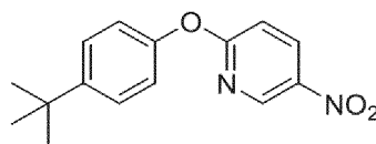
Formula (IIa)
