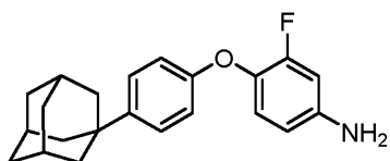
4-((3r,5r,7r)-Adamantan-1-yl)phenoxy-3-fluoroaniline,
