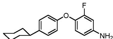
4-(4-Cyclohexylphenoxy)-3-fluoroaniline,
