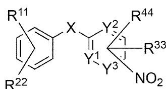
Formula (II)
