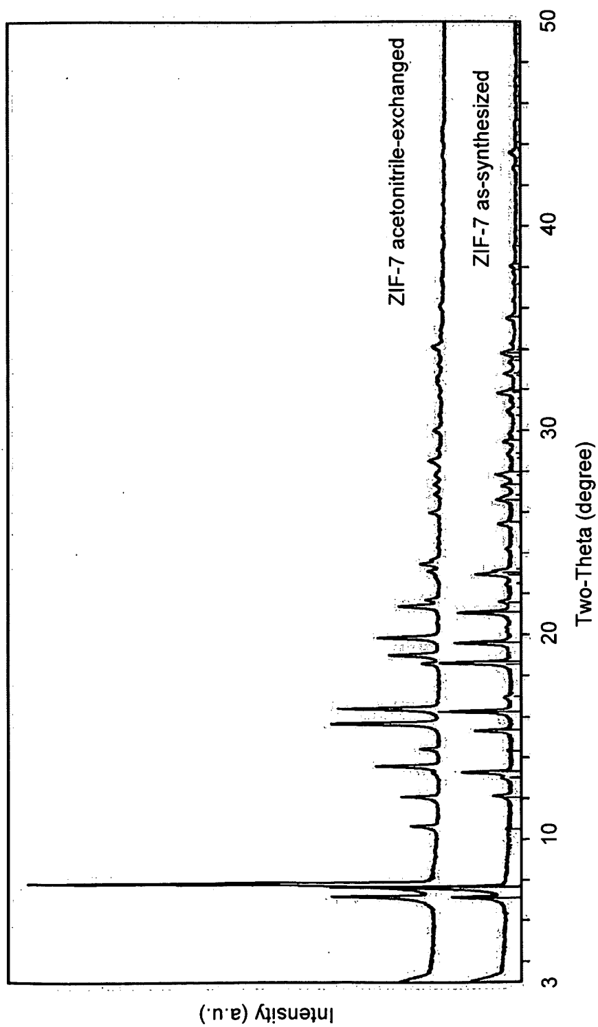
Powder X-ray Diffraction Pattern of ZIF-7
