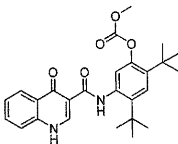
Compound 33
