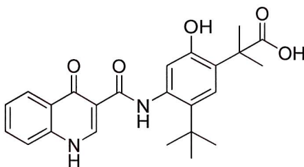
Compound 28
