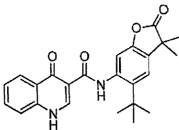
Compound 21
