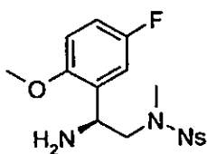
N-[(2S)-2-amino-2-(5-fluoro-2-methoxyphenyl)ethyl]-N-methyl-4-nitrobenzenesulfonamide (6)
