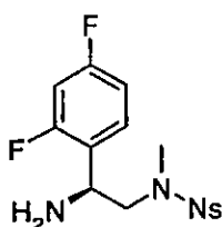
(S)-N-(2-amino-2-(2,4-difluorophenyl)ethyl)-N-methyl-4-nitrobenzenesulfonamide (42)
