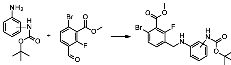
Scheme 10
