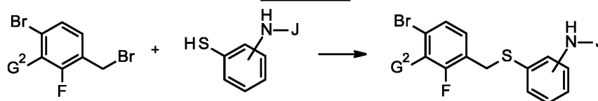
Scheme 13
