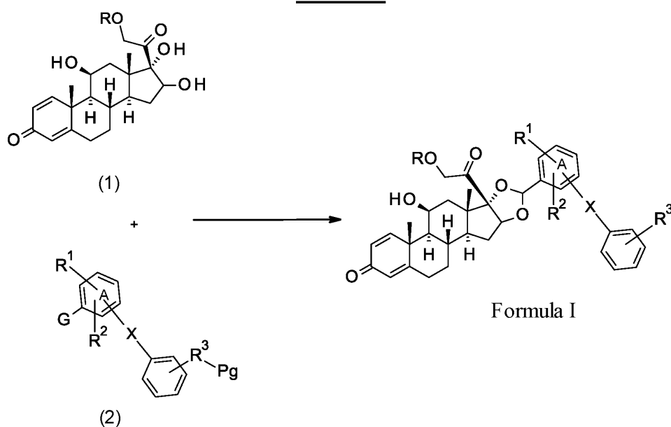
Scheme 17
