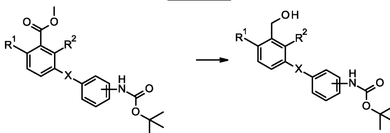
Scheme 11
