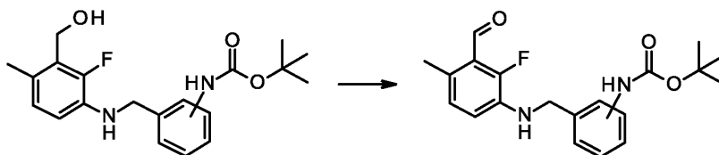
Scheme 15
