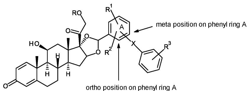
Formula I
