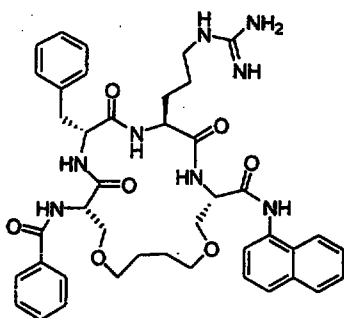
12-Benzoylamino-9-benzyl-6-(3-guanidino-propyl)- 5,8,11-trioxo-1,14-dioxo-4,7,10-triaza- cyclooctadecane-3-carboxylic acid naphthalen-1- ylamide
