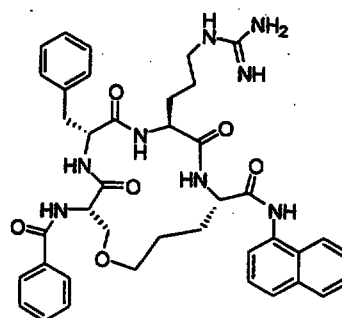
3-Benzoylamino-6-benzyl-9-(3-guanidino-propyl)- 4,7,10-trioxo-1-oxa-5,8,11-triaza- cyclopentadecane-12-carboxylic acid naphthalen-1- ylamide
