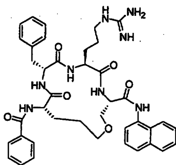
12-Benzoylamino-9-benzyl-6-(3-guanidino-propyl)- 5,8,11-trioxo-1-oxa-4,7,10-triaza- cyclopentadecane-3-carboxylic acid naphthalen-1- ylamide
