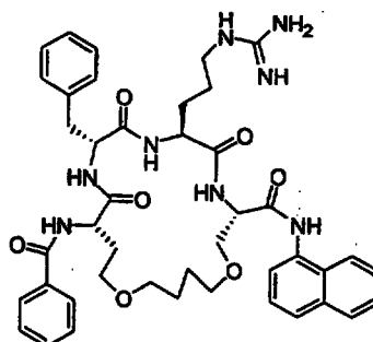
12-Benzoylamino-9-benzyl-6-(3-guanidino-propyl)- 5,8,11-trioxo-1,15-dioxo-4,7,10-triaza- cyclononadecane-3-carboxylic acid naphthalen-1- ylamide
