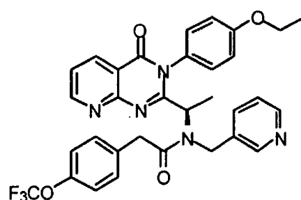
(+)-(S)-N-{1-[3-(4-Ethoxy-phenyl)-4-oxo-3,4-dihydro-pyrido[2,3-d]pyrimidin-2-yl]-ethyl}-N-pyridin-3-yl methyl-2-(4-trifluoromethoxy-phenyl)-acetamide
