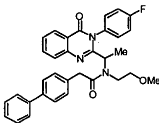
2-Biphenyl-4-yl- N-(1-[3-(4-fluoro-phenyl)-4-oxo-3,4-dihydro-quinazolin-2-yl]-ethyl)- N-(2-methoxy-ethyl)-acetamide (1.17)
