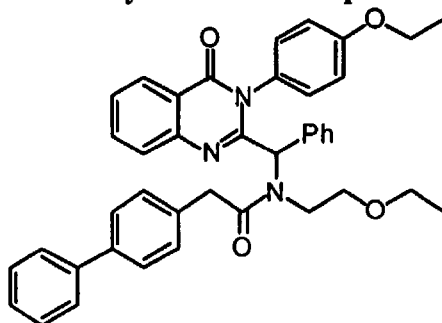
2-Biphenyl-4-yl- N -(2-ethoxy-ethyl)- N -[[3-(4-ethoxy-phenyl)-4-oxo-3,4-dihydro-quinazolin-2-yl]-phenyl-methyl]-acetamide 1.51
