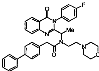
2-Biphenyl-4-yl-N-{1-[3-(4-fluoro-phenyl)-4-oxo-3,4-dihydro-quinazolin-2-yl]-ethyl}-N-(2-morpholin-4-yl-ethyl)-acetamide (1.18)
