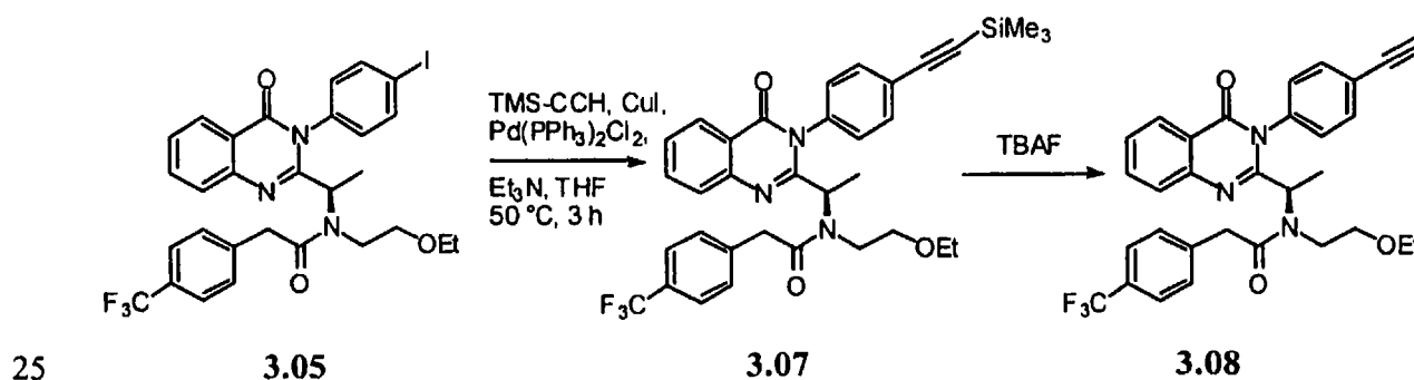
Scheme 7
