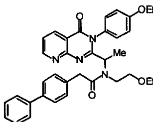
2-Biphenyl-4-yl-N-(2-ethoxy-ethyl)-N-(1-[3-(4-ethoxy-phenyl)-4-oxo-3,4-dihydro-pyrido[2,3-d]pyrimidin-2-yl]-ethyl)-acetamide (2.10)
