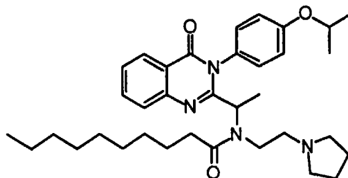
Decanoic acid {1-[3-(4-isopropoxyphenyl)-4-oxo-3,4-dihydro-quinazolin-2-yl]-ethyl}-(2-pyrrolidin-1-yl-ethyl)-amide
