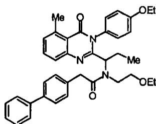
2-Biphenyl-4-yl-N-(2-ethoxy-ethyl)-N-(1-[3-(4-ethoxy-phenyl)-5-methyl-4-oxo-3,4-dihydro-quinazolin-2-yl]-propyl)-acetamide (2.11)
