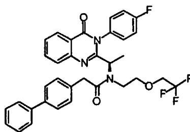
2-Biphenyl-4-yl-N-{1-[3-(4-fluoro-phenyl)-4-oxo-3,4-dihydro-quinazolin-2-yl]-ethyl}-N-[2-(2,2,2-trifluoro-ethoxy)-ethyl]-acetamide
