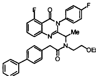
2-Biphenyl-4-yl-N-(2-ethoxy-ethyl)-N-(1-[5-fluoro-3-(4-fluoro-phenyl)-4-oxo-3,4-dihydro-quinazolin-2-yl]-ethyl)-acetamide (2.06)
