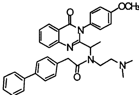
2-Biphenyl-4-yl-N-(2-dimethylamino-ethyl)-N-{1-[3-(4-methoxyphenyl)-4-oxo-3,4-dihydro-quinazolin-2-yl]-ethyl}-acetamide
