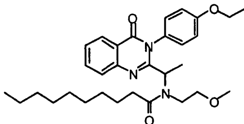
Decanoic acid {1-[3-(4-ethoxy-phenyl)-4-oxo-3,4-dihydro-quinazolin-2-yl]-ethyl}-(2-methoxy-ethyl)-amide 1.32
