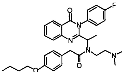
2-(4-Butoxy-phenyl)-N-(2-dimethylamino-ethyl)-N-{1-[ 3-(4-fluoro-phenyl)-4-oxo-3,4-dihydro-quinazolin-2-yl]-ethyl}-acetamide
