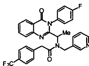
N -{1-[3-(4-Fluoro-phenyl)-4-oxo-3,4-dihydro-quinazolin-2-yl]-ethyl}- N -pyridin-3-ylmethyl-2-(4-trifluoromethyl-phenyl)-acetamide (1.27)
