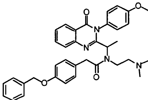
2-(4-Benzyloxy-phenyl)-N-(2-dimethylamino-ethyl)- N-{1-[3-(4-methoxy-phenyl)-4-oxo-3,4-dihydro-qu inazolin-2-yl]-ethyl}-acetamide
