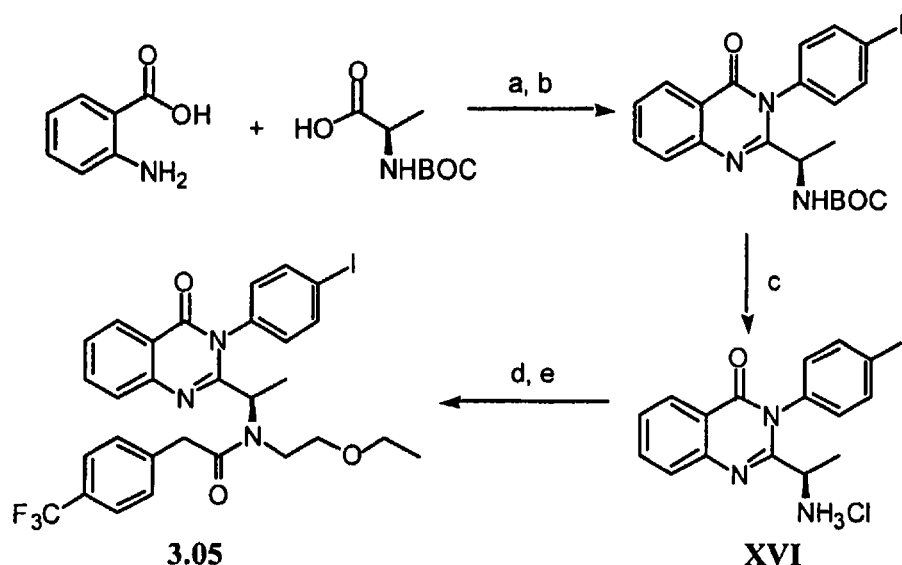
Scheme 5
