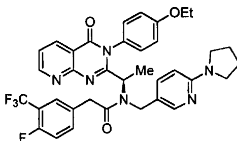
(R) -N-{1-[3-(4-Ethoxy-phenyl)-4-oxo-3,4-dihydro-pyrido[2,3- d ]pyrimidin-2-yl]-ethyl}-2-(4-fluoro-3-trifluoromethyl-phenyl)-N-(6-pyrrolidin-1-yl-pyridin-3-ylmethyl)-acetamide
