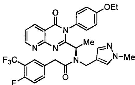
(R)-N-{1-[3-(4-Ethoxy-phenyl)-4-oxo-3,4-dihydro-pyrido[2,3-d]pyrimidin-2-yl]-ethyl}-2-(4-fluoro-3-trifluoromethyl-phenyl)-N-(1-methyl-1H-pyrazol-4-ylmethyl)-acetamide
