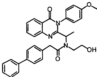
2-Biphenyl-4-yl-N-(2-hydroxy-ethyl)-N-{1-[3-(4-methoxy-phenyl)-4-oxo-3,4-dihydro-quinazolin-2-yl]-ethyl}-acetamide
