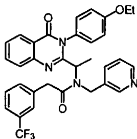
N -{1-[3-(4-Ethoxy-phenyl)-4-oxo-3,4-dihydro-quinazolin-2-yl]-ethyl}- N -pyridin-3-ylmethyl-2-(3-trifluoromethyl-phenyl)-acetamide
