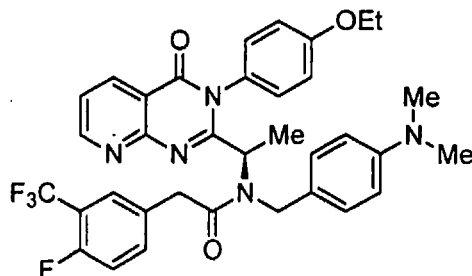
( R )- N -(4-Dimethylamino-benzyl)- N -{1-[3-(4-ethoxy-phenyl)-4-oxo-3,4-dihydro-pyrido[2,3- d ]pyrimidin-2-yl]-ethyl}-2-(4-fluoro-3-trifluoromethyl-phenyl)-acetamide
