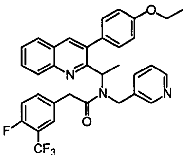
N-{1-[3-(4-Ethoxy-phenyl)-quinolin-2-yl]-ethyl}-2-(4-fluoro-3-trifluoromethyl-phenyl)-N-pyridin-3-ylmethyl-acetamide
