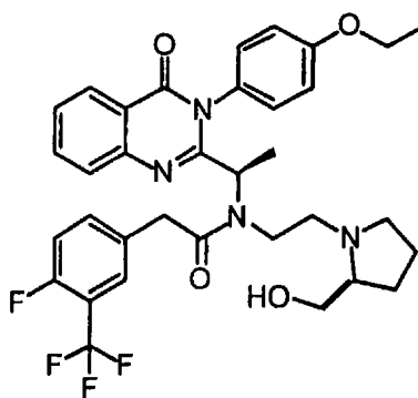
(s)-N-{1-[3-(4-Ethoxy-phenyl)-4-oxo-3,4-dihydro-quinazolin-2-yl]-ethyl}-2-(4-fluoro-3-trifluoromethyl-phenyl)-N-[2-(2-hydroxymethyl-pyrrolidin-1-yl)-ethyl]-acetamide 3.37
