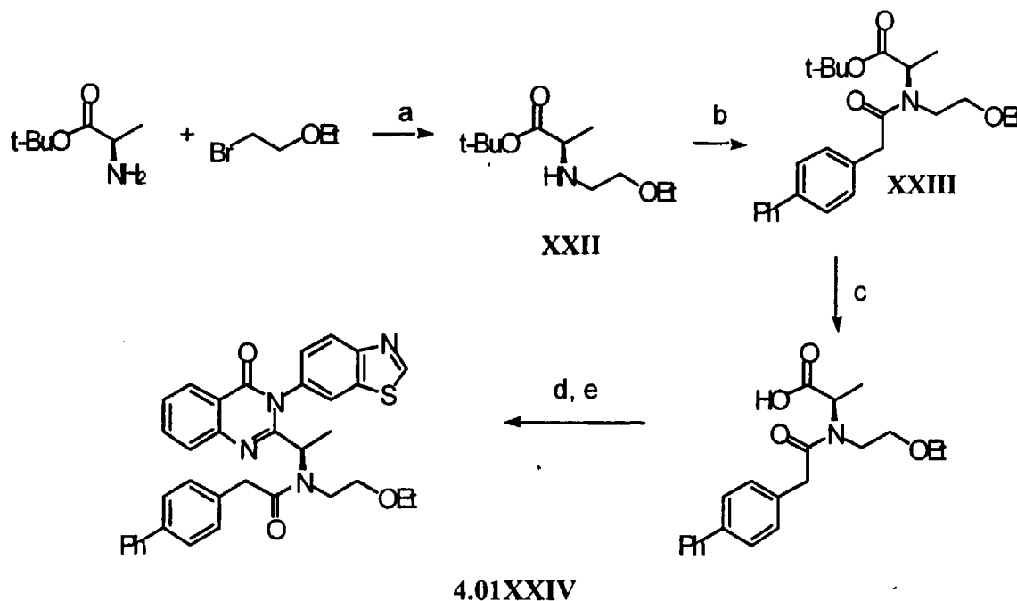
Scheme 12
