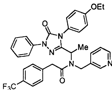
N -{1-[4-(4-Ethoxy-phenyl)-5-oxo-1-phenyl-4,5-dihydro-1H-[1,2,4]triazol-3-yl]-ethyl}- N -pyridin-3-ylmethyl-2-(4-trifluoromethyl-phenyl)-acetamide
