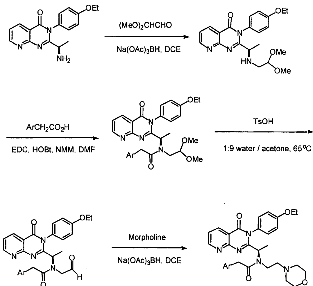
Scheme 11
