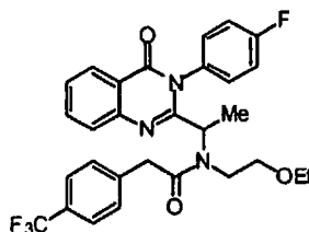
N -(2-Ethoxy-ethyl)- N -{1-[3-(4-fluoro-phenyl)-4-oxo-3,4-dihydro-quinazolin-2-yl]-ethyl}-2-(4-trifluoromethyl-phenyl)-acetamide (1.26)
