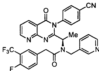
(R)-N-{1-[3-(4-Cyano-phenyl)-4-oxo-3,4-dihydro-pyrido[2,3-d]pyrimidin-2-yl]-ethyl}-2-(4-fluor-3-trifluoro methyl-phenyl)-N-pyridin-3-ylmethyl-acetamide
