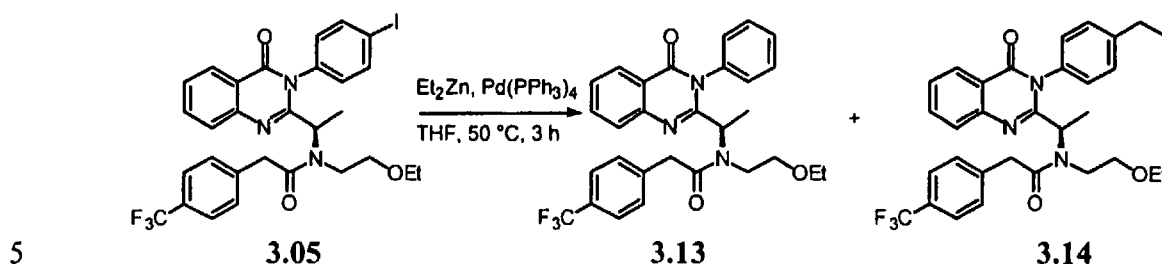
Scheme 8
