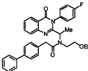
2-Biphenyl-4-yl-N-(2-ethoxy-ethyl)-N-{1-[3-(4-fluoro-phenyl)-4-oxo-3,4-dihydro-quinazolin-2-yl]-ethyl}-acetamide (1.19)
