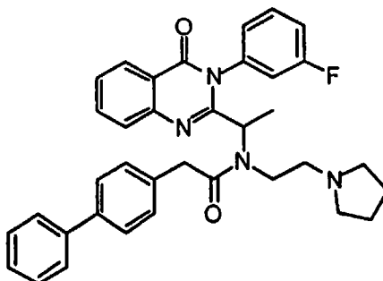
2-Biphenyl-4-yl- N -{1-[3-(3-fluoro-phenyl)-4-oxo-3,4-dihydro-quinazolin-2-yl]-ethyl}- N -(2-pyrrolidin-1-yl-ethyl)-acetamide
