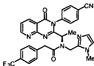
(1R-[3-(4-Cyano-phenyl)-4-oxo-3,4-dihydro-pyrido[2,3-d]rimidin-2-yl]-ethyl)-N-(1-methyl-1H-imidazol-2-ylmethyl)-2-(4-trifluoromethyl-phenyl)-acetamide ( 3.21)
