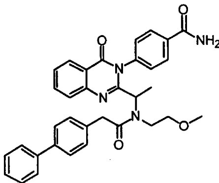
4-(2-{1-[(Biphenyl-4-yl-acetyl)-(2-methoxy-ethyl)-amino]-ethyl}-4-oxo-4H-quinazolin-3-yl)-benzamide
