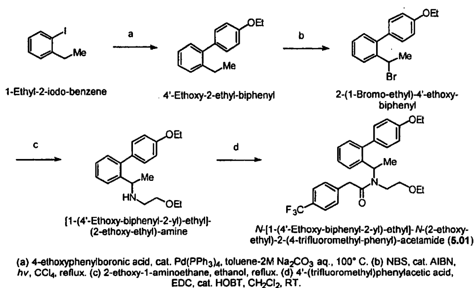
Scheme 13
