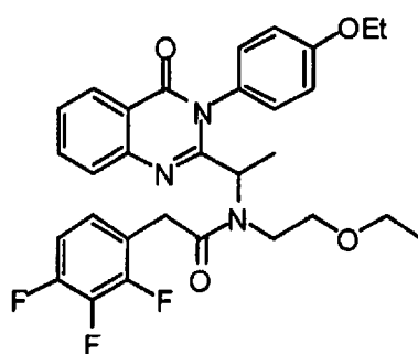
N -Ethoxymethyl- N -{1-[3-(4-ethoxy-phenyl)-4-oxo-3,4-dihydro-quinazolin-2-yl]-ethyl}-2-(2,3,4-trifluoro-phenyl)-acetamide
