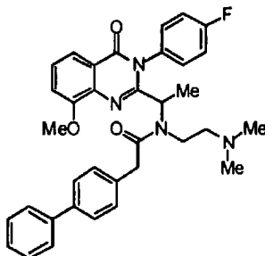
2-Biphenyl-4-yl- N -(2-dimethylamino-ethyl)- N -(1-[3-(4-fluoro-phenyl)-8-methoxy-4-oxo-3,4-dihydro-quinazolin-2-yl]-ethyl)-acetamide (2.02)
