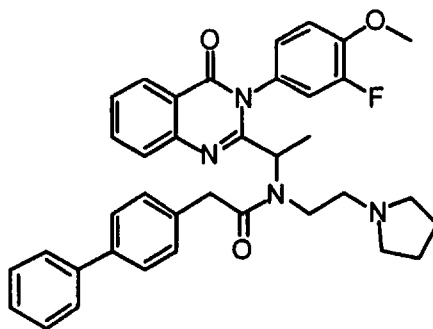
2-Biphenyl-4-yl-N-{1-[3-(3-fluoro-4-methoxy-phenyl)-4-oxo-3,4-dihydro-quinazolin-2-yl]-ethyl}-N-(2-pyrrolidin-1-yl-ethyl)-acetamide 1.33
