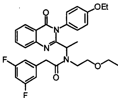
2-(3,5-Difluoro-phenyl)- N -(2-ethoxy-ethyl)- N -(1-[3-(4-ethoxy-phenyl)-4-oxo-3,4-dihydro-quinazolin-2-yl]-ethyl)-acetamide
