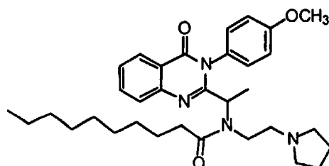
Decanoic acid {1-[3-(4-methoxy-phenyl)-4-oxo-3,4-dihydro-quinazolin-2-yl]-ethyl}-(2-pyrrolidin-1-yl-ethyl)-amide
