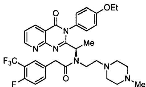
(R) -N-{1-[3-(4-Ethoxy-phenyl)-4-oxo-3,4-dihydro-pyrido[2,3- d ]pyrimidin-2-yl]-ethyl}-2-(4-fluoro-3-trifluoromethyl-phenyl)-N-[2-(4-methyl-piperazin-1-yl)-ethyl]-acetamide
