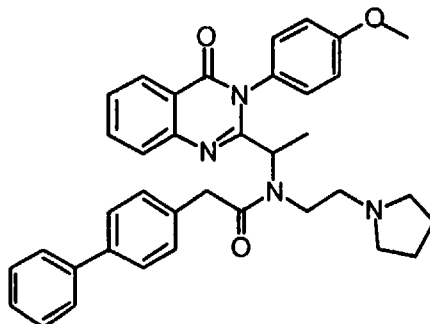
2-Biphenyl-4-yl- N -{1-[3-(4-methoxy-phenyl)-4-oxo-3,4-dihydro-quinazolin-2-yl]-ethyl}- N -(2-pyrrolidin-1-yl-ethyl)-acetamide
