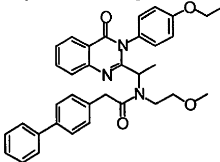
2-Biphenyl-4-N-{1-[3-(4-ethoxy-phenyl)-4-oxo-3,4 ro-quinazolin-2-yl]-N-(2-ethoxy-ethyl)-
