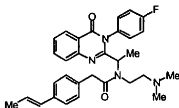
N -(2-Dimethylamino-ethyl)- N -(1-[3-(4-fluoro-phenyl)-4-oxo-3,4-dihydro-quinazolin-2-yl]-ethyl)-2-(4- E -propenyl-phenyl)-acetamide (1.14)
