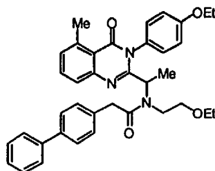
2-Biphenyl-4-yl-N-(2-ethoxy-ethyl)-N-{1-[3-(4-ethoxy-phenyl)-5-methyl-4-oxo-3,4-dihydro-quinazolin-2-yl]-ethyl}-acetamide (2.08)
