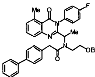
2-Biphenyl-4-yl-N-(2-ethoxy-ethyl)-N-(1-[5-methyl-3-(4-fluoro-phenyl)-4-oxo-3,4-dihydro-quinazolin-2-yl]-ethyl)-acetamide (2.07)
