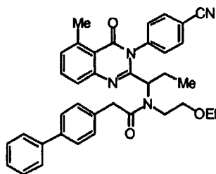
2-Biphenyl-4-yl-N-(2-ethoxy-ethyl)-N-{1-[3-(4-cyano-phenyl)-5-methyl-4-oxo-3,4-dihydro-quinazolin-2-yl]-propyl}-N-(2-ethoxy-ethyl)-acetamide (2.09)
