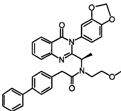
N -[1-(3-Benzo[1,3]dioxol-5-yl-4-oxo-3,4-dihydro-quinazolin-2-yl)-ethyl]-2-biphenyl-4-yl- N -(2-methoxy-ethyl)-acetamide
