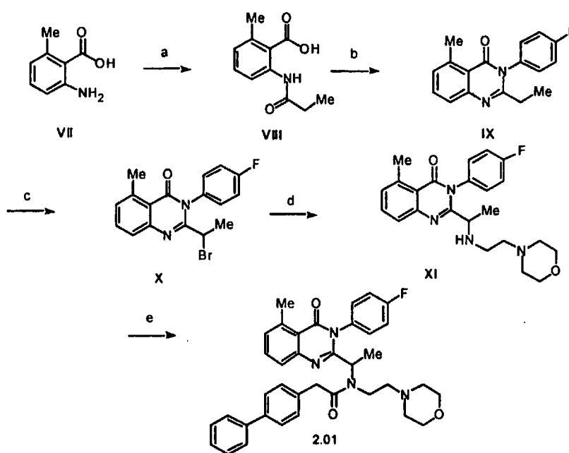
Scheme 2
