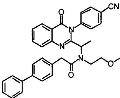
2-Biphenyl-4-yl- N -{1-[3-(4-cyano-phenyl)-4-oxo-3,4-dihydro-quinazolin-2-yl]-ethyl}- N -(2-methoxy-ethyl)-acetamide
