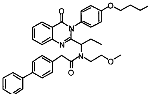
2-Biphenyl-4-yl-N-{1-[3-(4-butoxy-p henyl)-4-oxo-3,4-dihydro-quinazolin -2-yl]-propyl}-N-(2-methox y-ethyl)-acetamide 1.40
