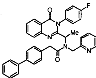
2-Biphenyl-4-yl-N-{1-[3-(4-fluoro-phenyl)-4-oxo-3,4-dihydro-quinazolin-2-yl]-ethyl}-N-pyridin-2-ylmethyl-acetamide ( 1.22 )
