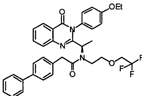
2-Biphenyl-4-yl-N-{1-[3-(4-ethoxy-phenyl)-4-oxo-3,4-dihydro-quinazolin-2-yl]-ethyl}-N-[2-(2,2,2-trifluoro-ethoxy)-ethyl]-acetamide
