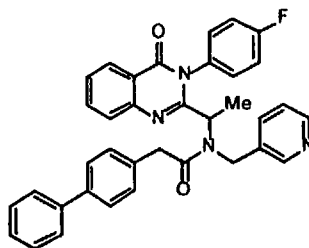
2-Biphenyl-4-yl- N-[1-[3-(4-fluoro-phenyl)-4-oxo-3,4-dihydro-quinazolin-2-yl]-ethyl]- N-pyridin-3-ylmethyl-acetamide (1.23)
