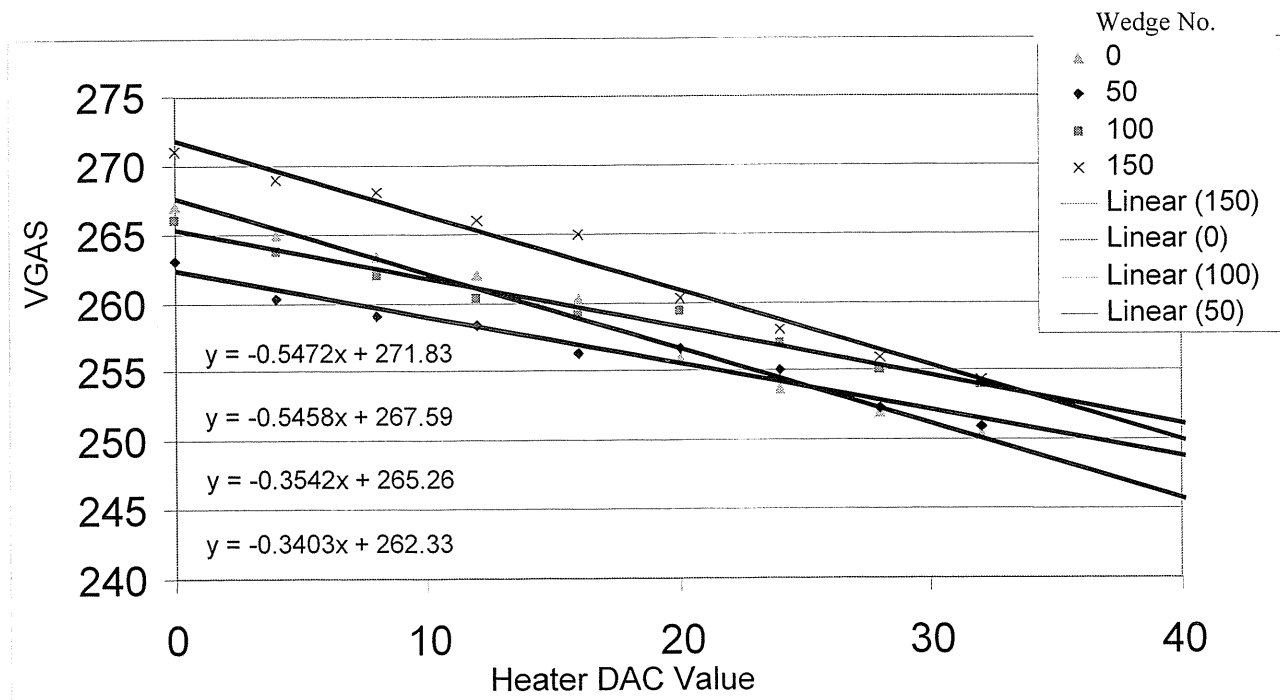
VGAS to Read Heater Characterization at Wedge (0, 50, 100, 150)
