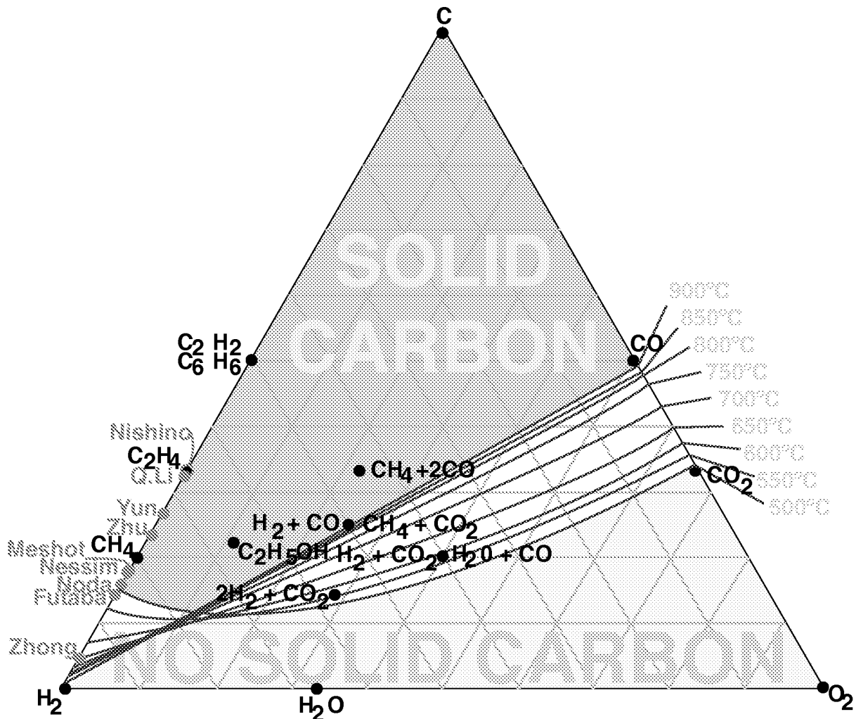
C-H-O EQUILIBRIUM DIAGRAM equilibrium lines show the cutoff for solid carbon information at each temperature
