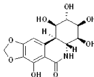
Pancratistatin 2
