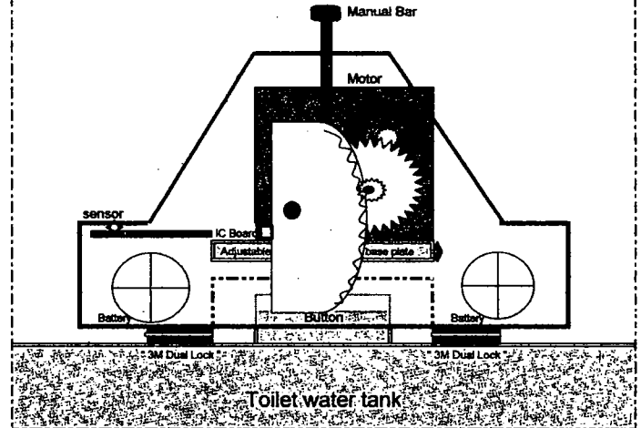
(E) Round Gear system
