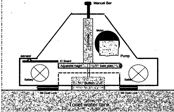
(B) Hydraulic system
