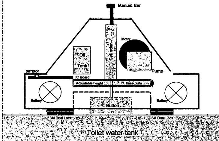
(C) Water Jack system
