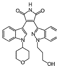
Compound 14a
