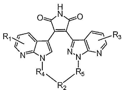
Formula (IIIg)
