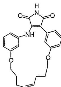
Compound 14a
