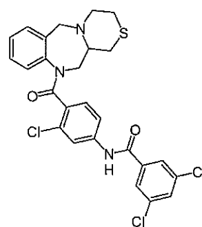
Compound 3a
