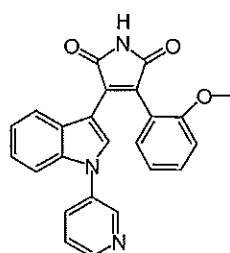
Compound 2a
