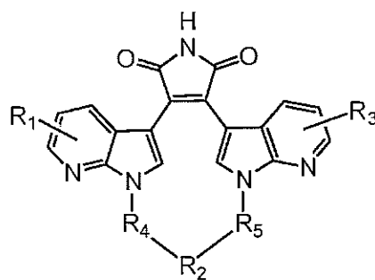
Formula (IIIb)
