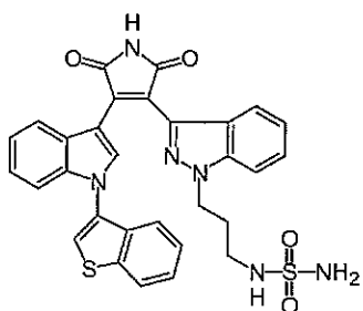
Compound 10a
