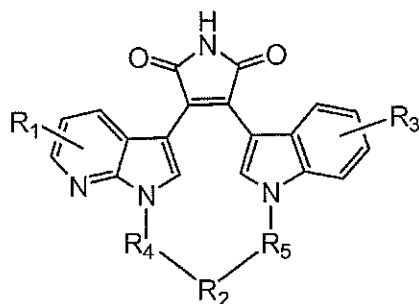
Formula (IIIj)
