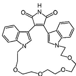
Compound 6
