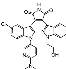
Compound 31a
