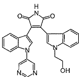
Compound 10a
