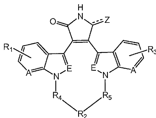
Formula (III)
