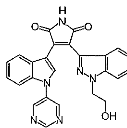
Compound 12a
