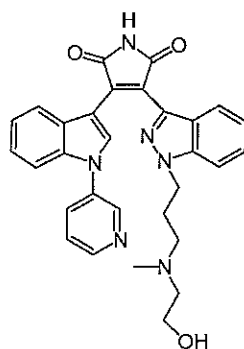
Compound 2a
