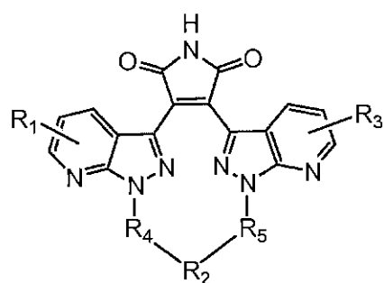
Formula (IIId)
