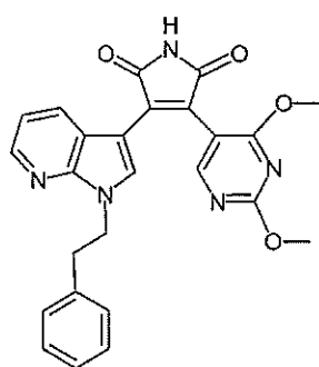
Compound 44
