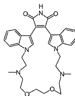
Compound 24a
