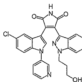
Compound 12a
