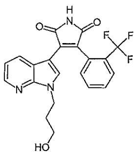
Compound 11
