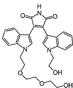
Compound 19a
