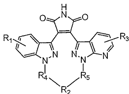
Formula (IIIIm)
