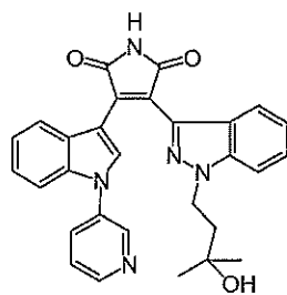
Compound 11a
