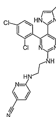
Compound 6a
