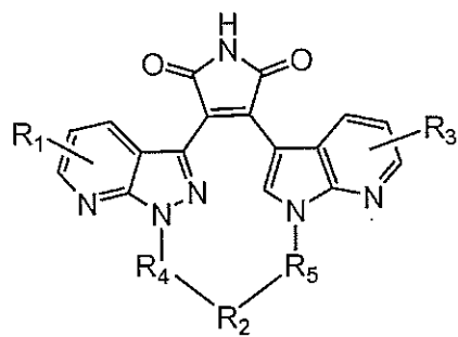
Formula (IIIh)
