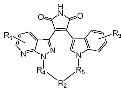
Formula (IIIl)
