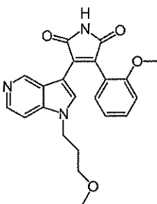
Compound 13a
