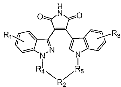
Formula (IIIe)
