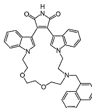
Compound 27a
