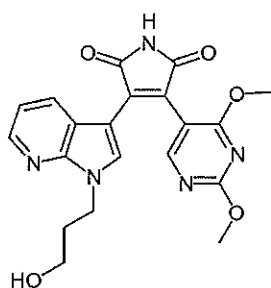
Compound 41
