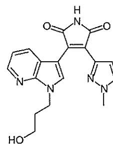
Compound 6a
