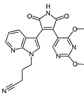
Compound 42
