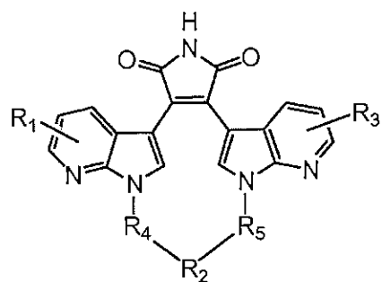
Formula (IIIb)
