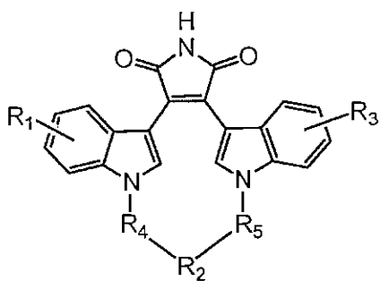
Formula (IIIa)
