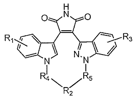
Formula (IIIf)
