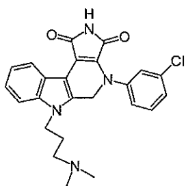
Compound 19a
