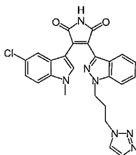
Compound 8a
