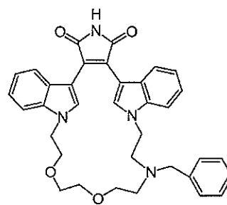
Compound 21a
