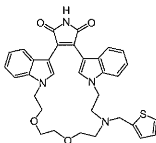
Compound 23a
