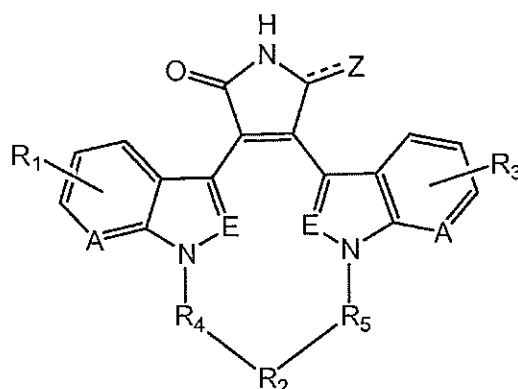
Formula (III)
