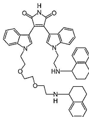
Compound 29a
