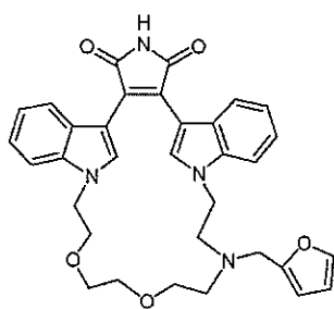
Compound 22a
