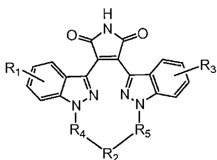
Formula (IIIc)
