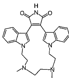
Compound 20a
