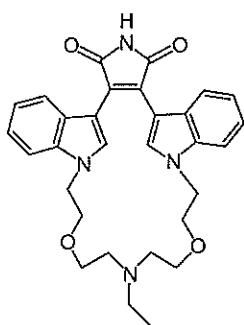
Compound 1a
