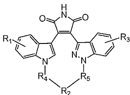
Formula (IIIf)
