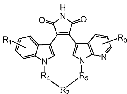
Formula (IIIi)
