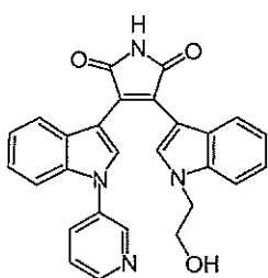
Compound 1a
