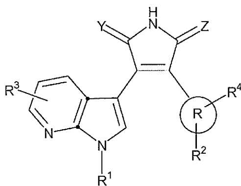
Formula (II)
