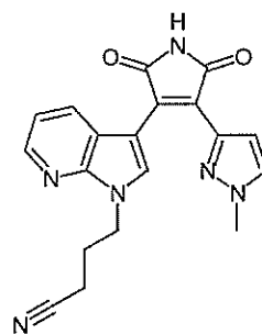
Compound 43
