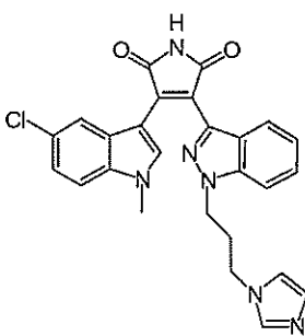
Compound 7a
