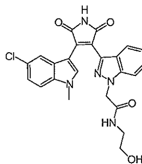
Compound 18a
