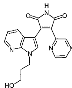
Compound 40
