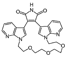
Compound 1
