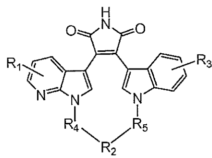
Formula (IIIj)
