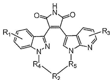
Formula (IIIIn)
