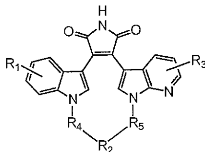
Formula (IIIi)
