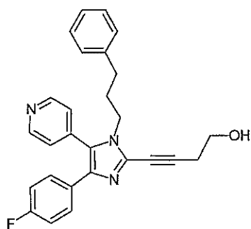
Compound 5.
