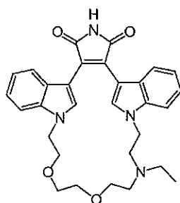
Compound 20a
