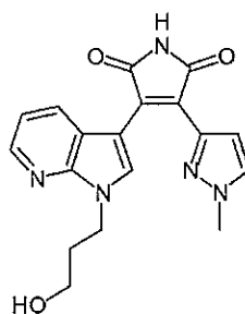
Compound 26
