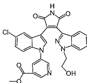
Compound 29a
