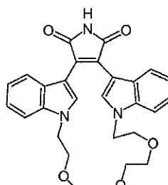
Compound 5
