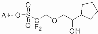
[Chemical Formula 3-11]
