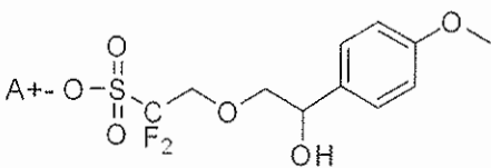
[Chemical Formula 3-12]
