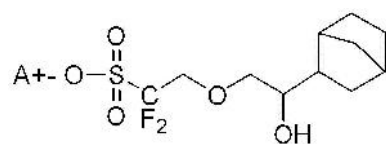
[Chemical Formula 3-4]
