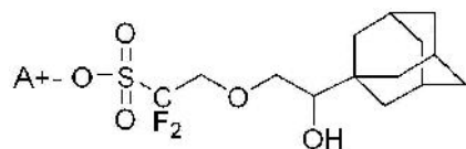
[Chemical Formula 3-2]
