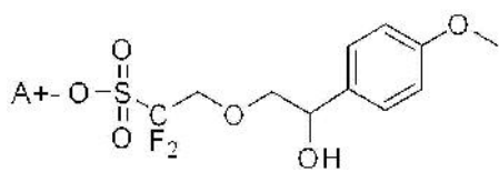
[Chemical Formula 3-12]
