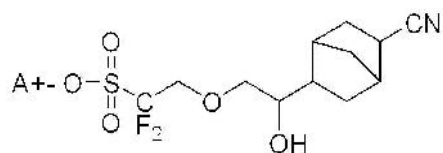
[Chemical Formula 3-10]
