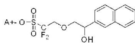
[Chemical Formula 3-6]
