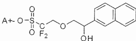
[Chemical Formula 3-5]
