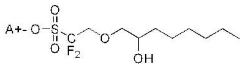
[Chemical Formula 3-12]
