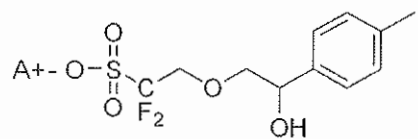
[Chemical Formula 3-7]
