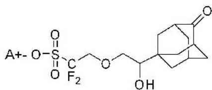
[Chemical Formula 3-8]
