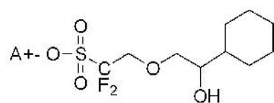
[Chemical Formula 3-3]
