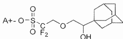
[Chemical Formula 3-2]
