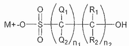
[Chemical Formula 7]
