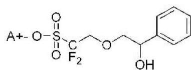
[Chemical Formula 3-5]
