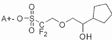
[Chemical Formula 3-11]
