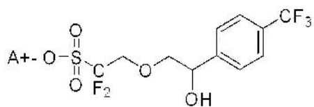
[Chemical Formula 3-9]
