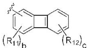
[Chemical Formula 2-1]
