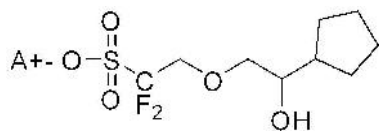
[Chemical Formula 3-11]
