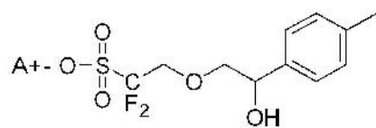
[Chemical Formula 3-7]
