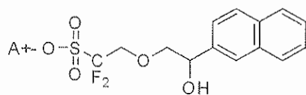
[Chemical Formula 3-6]
