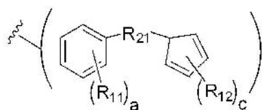
[Chemical Formula 2-1]
