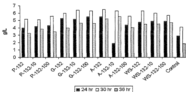
Chart 3B. Ethanol Concentrations for S. cerevisiae
